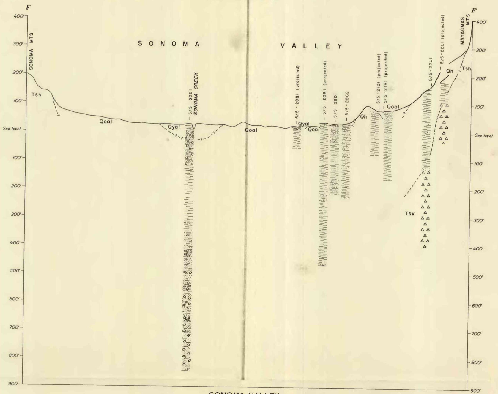
GEOLOGIC SECTIONS THROUGH NAPA AND SONOMA VALLEYS, CALIFORNIA
