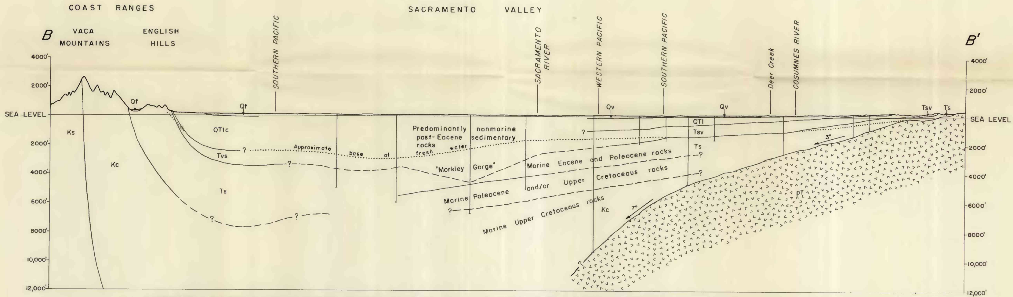
GENERALIZED GEOLOGIC SECTIONS A-A', B-B' ACROSS SACRAMENTO VALLEY, CALIFORNIA
