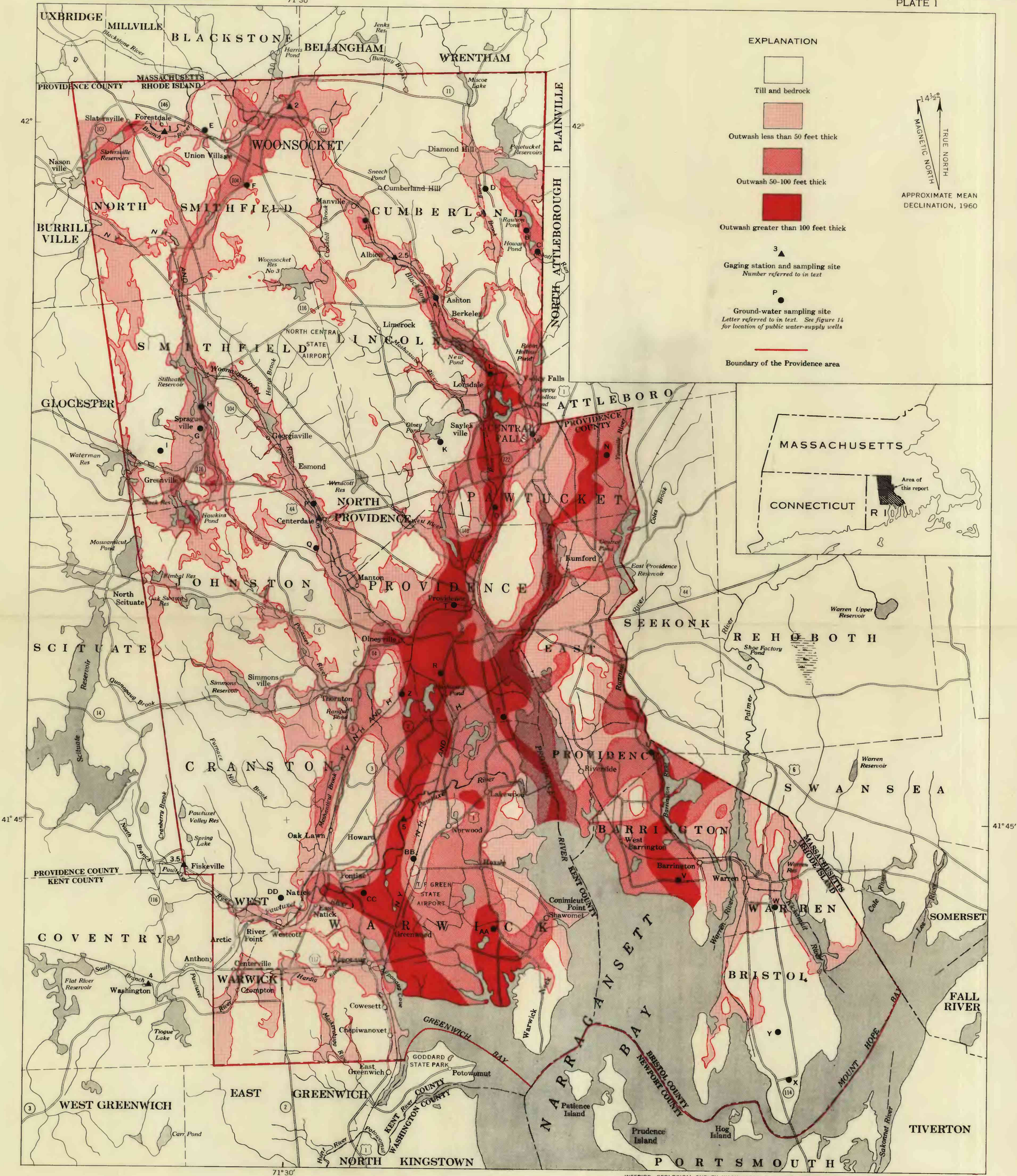
MAP OF THE PROVIDENCE AREA, RHODE ISLAND, SHOWING TILL AND BEDROCK, EXTENT AND THICKNESS OF OUTWASH, AND MEASURING AND SAMPLING SITES
