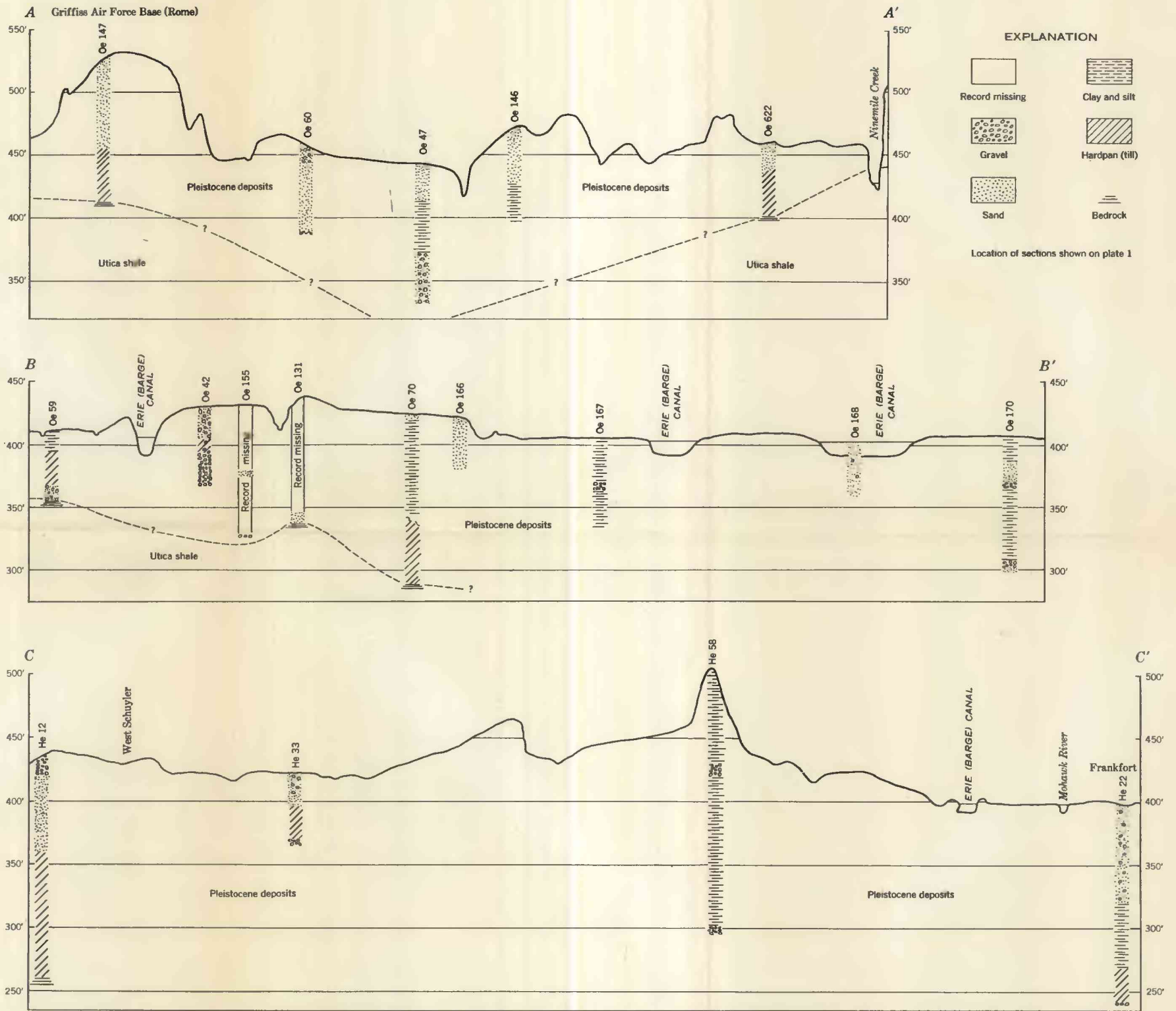
SECTIONS SHOWING UNCONSOLIDATED DEPOSITS IN THE MOHAWK RIVER CHANNEL BETWEEN ROME AND FRANKFORT
