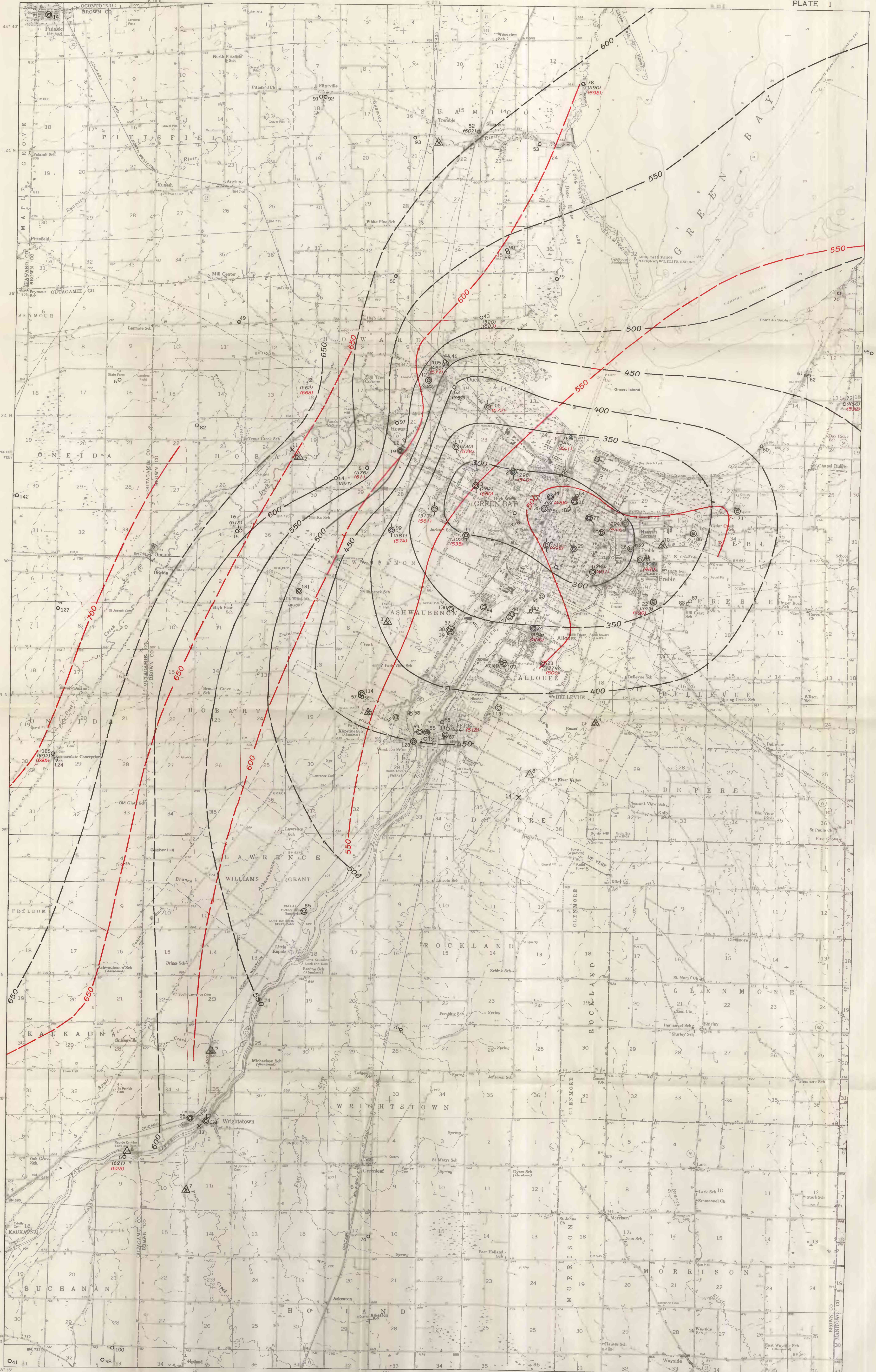
MAP OF GREEN BAY AREA, WISCONSIN, SHOWING THE PIEZOMETRIC SURFACE OF THE SANDSTONE AQUIFER IN AUGUST 1957 AND SEPTEMBER 1960, AND LOCATION OF WELLS, STREAMFLOW MEASURING SITES, AND SURFACE-WATER SAMPLING SITES
