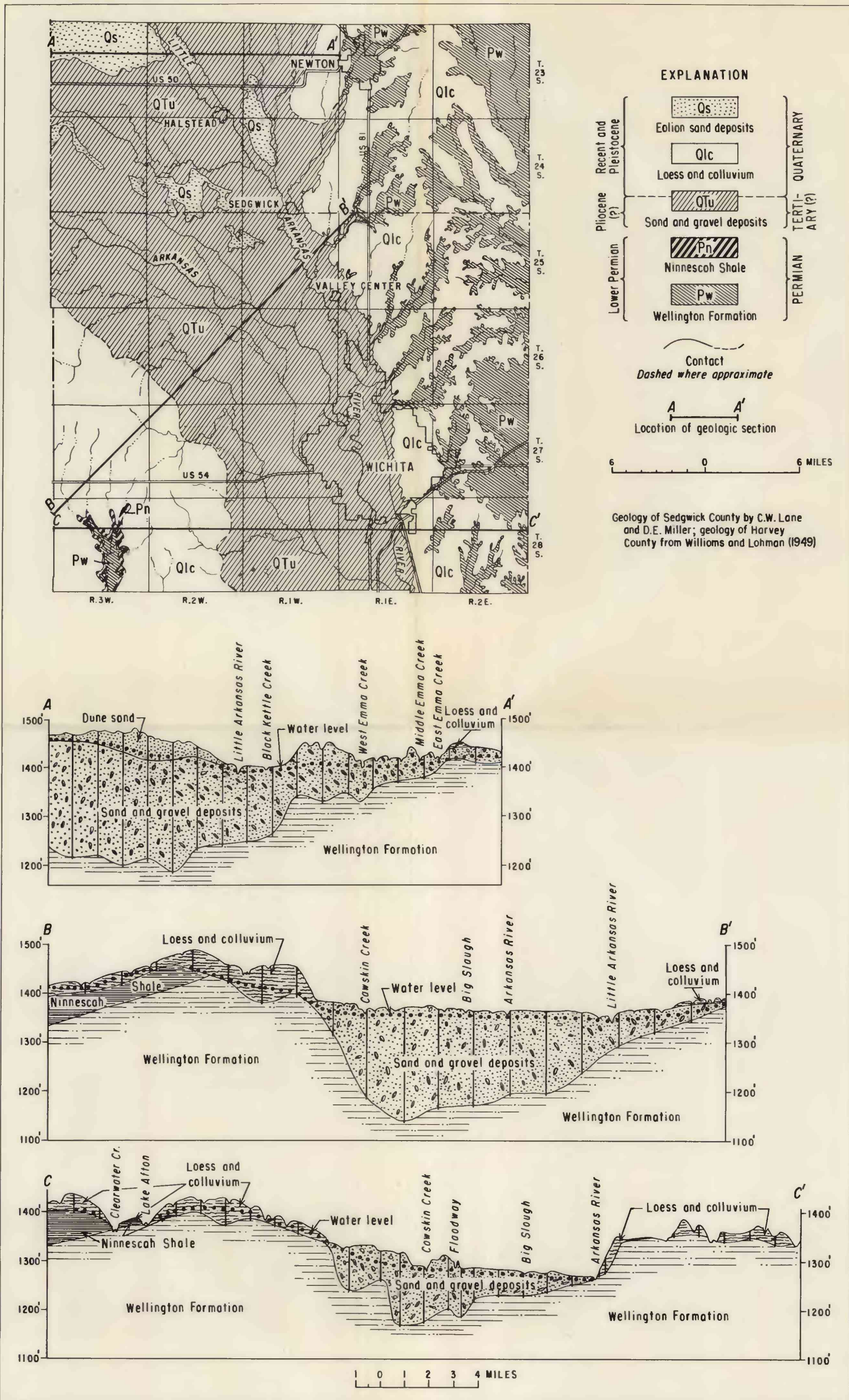
MAP SHOWING GENERALIZED AREAL GEOLOGY AND GENERALIZED GEOLOGIC SECTIONS, WICHITA AREA, KANSAS
