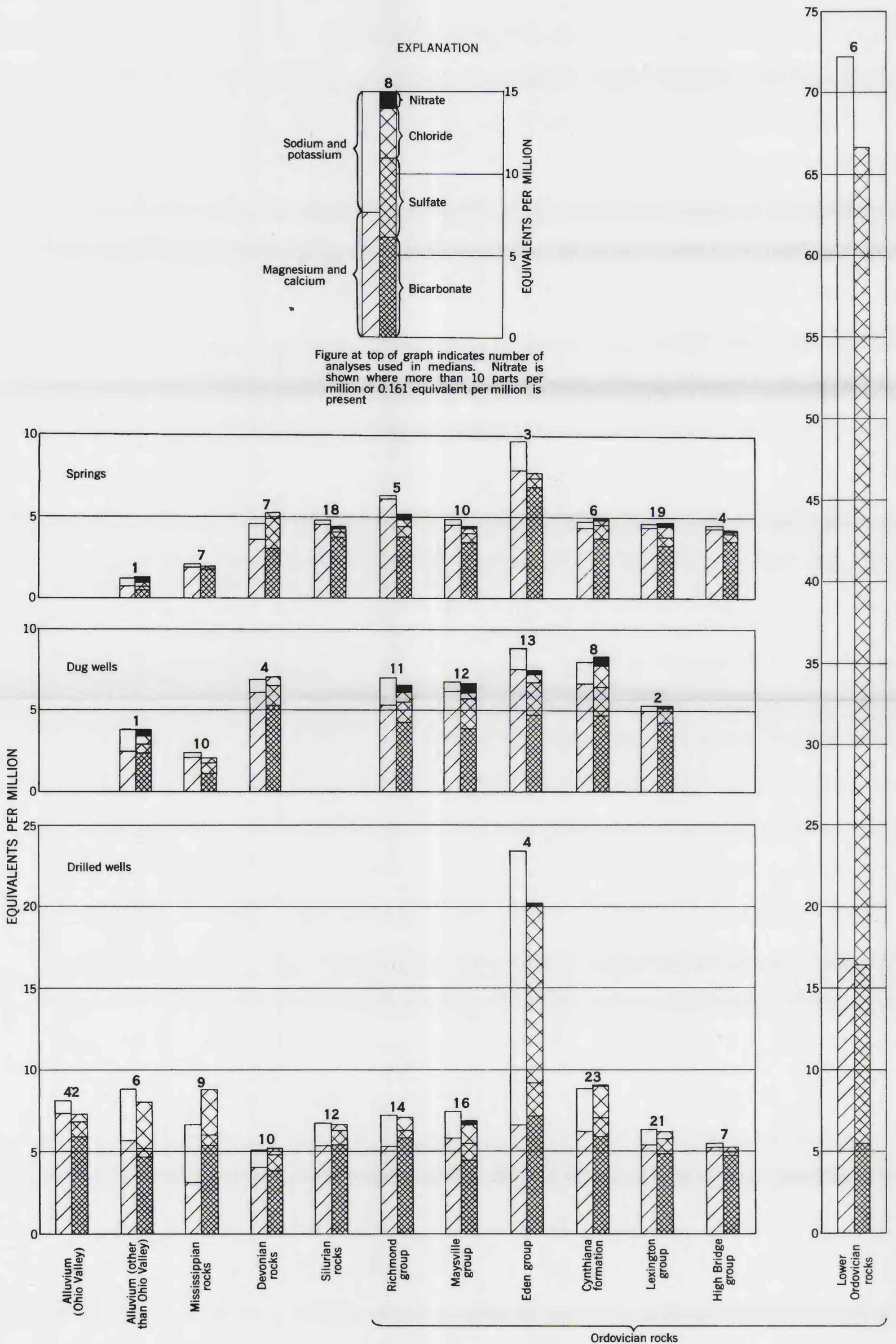
GRAPHS SHOWING MEDIAN VALUES, BY AQUIFERS, OF DISSOLVED CONSTITUENTS IN GROUND WATER IN THE BLUE GRASS REGION, KENTUCKY
