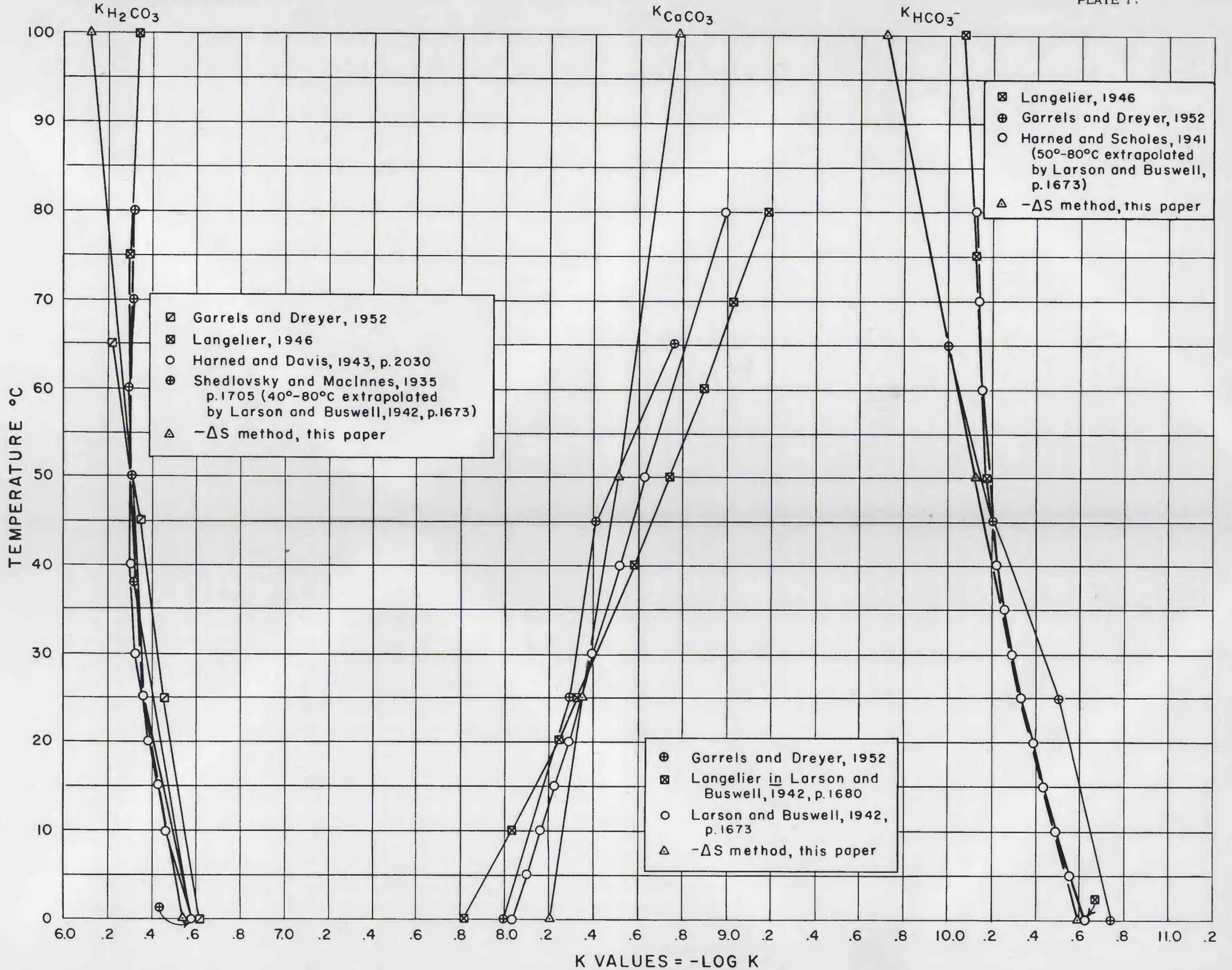
VALUES FOR EQUILIBRIUM CONSTANTS OBTAINED BY VARIOUS METHODS
