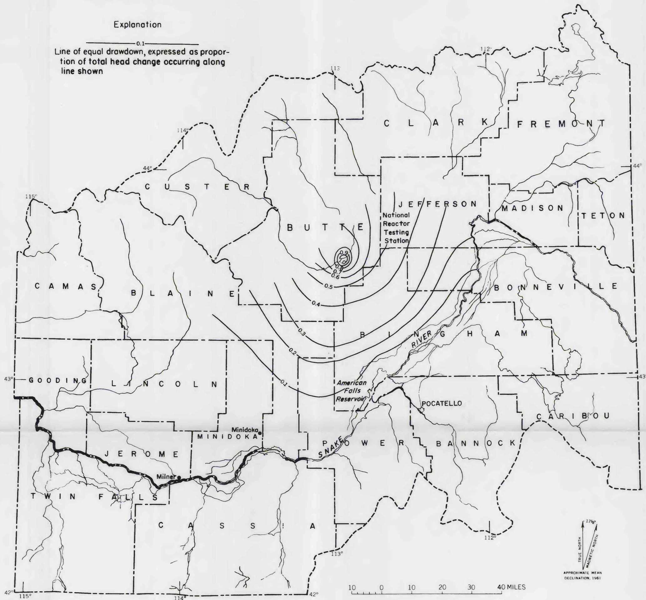
MAP SHOWING PREDICTED STABILIZED REGIONAL DRAWDOWN OF WATER TABLE CAUSED BY PUMPING AT NATIONAL REACTOR TESTING STATION, IDAHO (EFFECTS OF OTHER PUMPING IGNORED)
