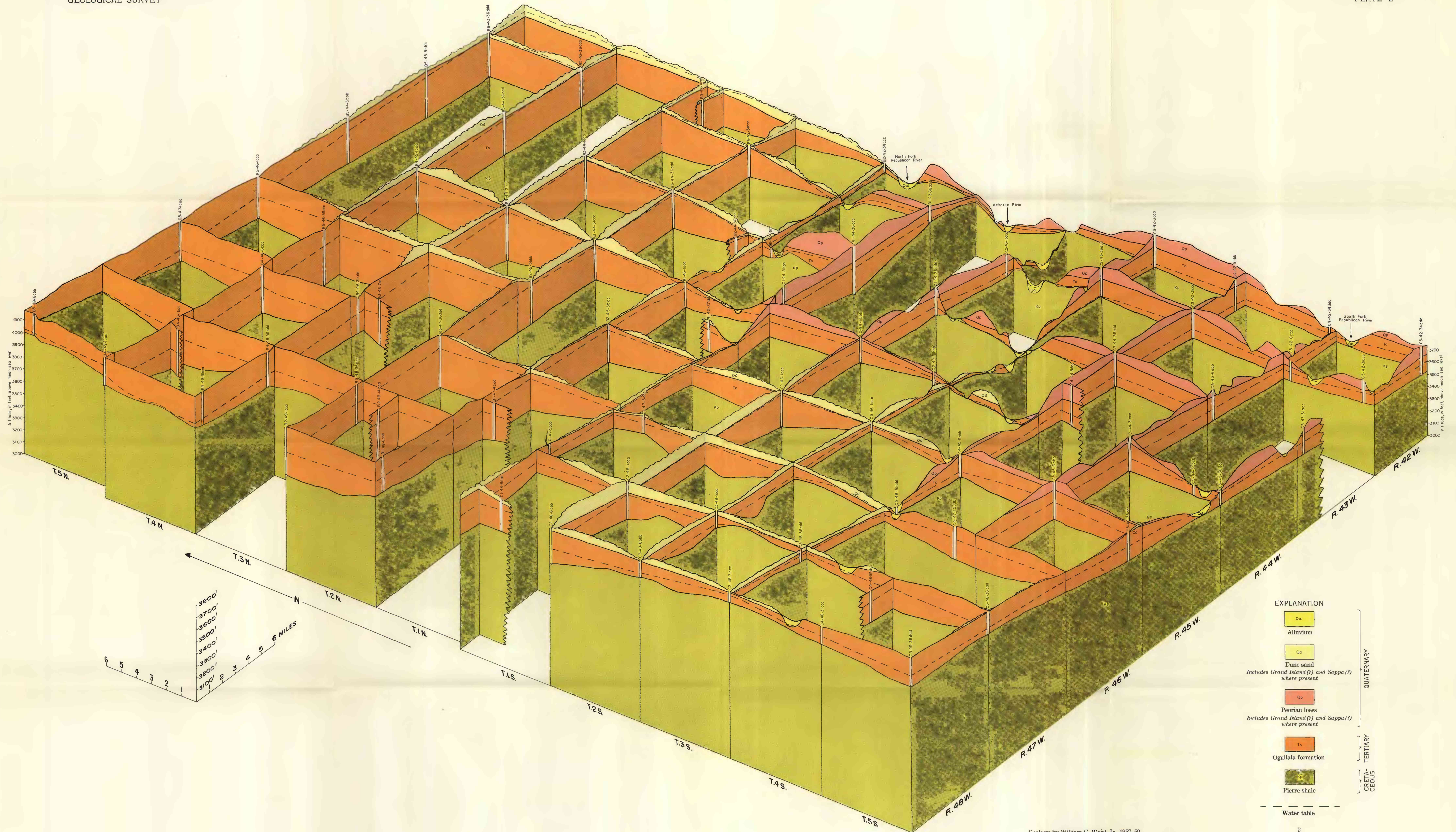
FENCE DIAGRAM OF YUMA COUNTY, COLORADO, SHOWING SUBSURFACE GEOLOGY
