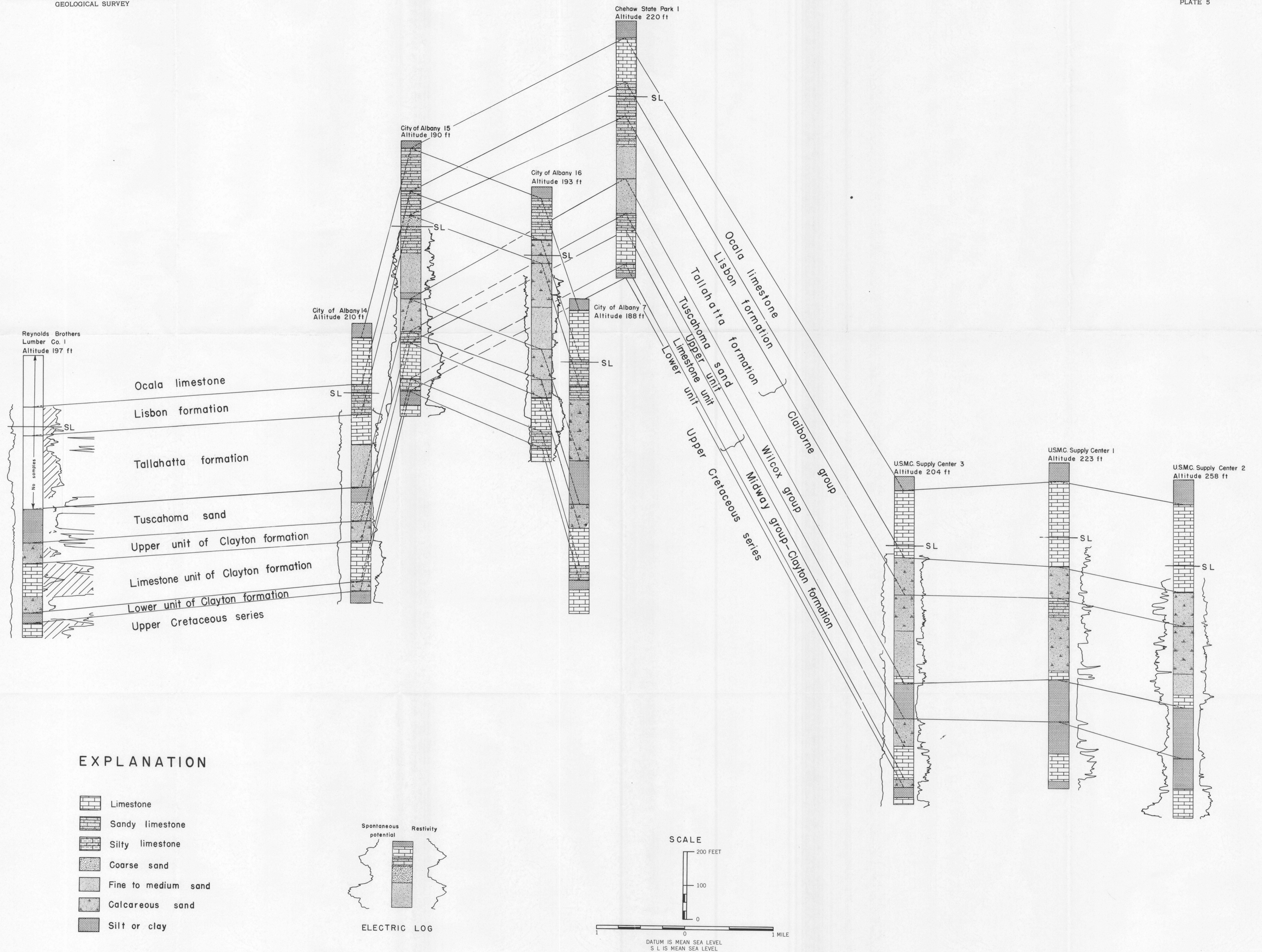
FENCE DIAGRAM SHOWING TERTIARY STRATIGRAPHY OF ALBANY, DOUGHERTY COUNTY, GEORGIA, AND VICINITY
