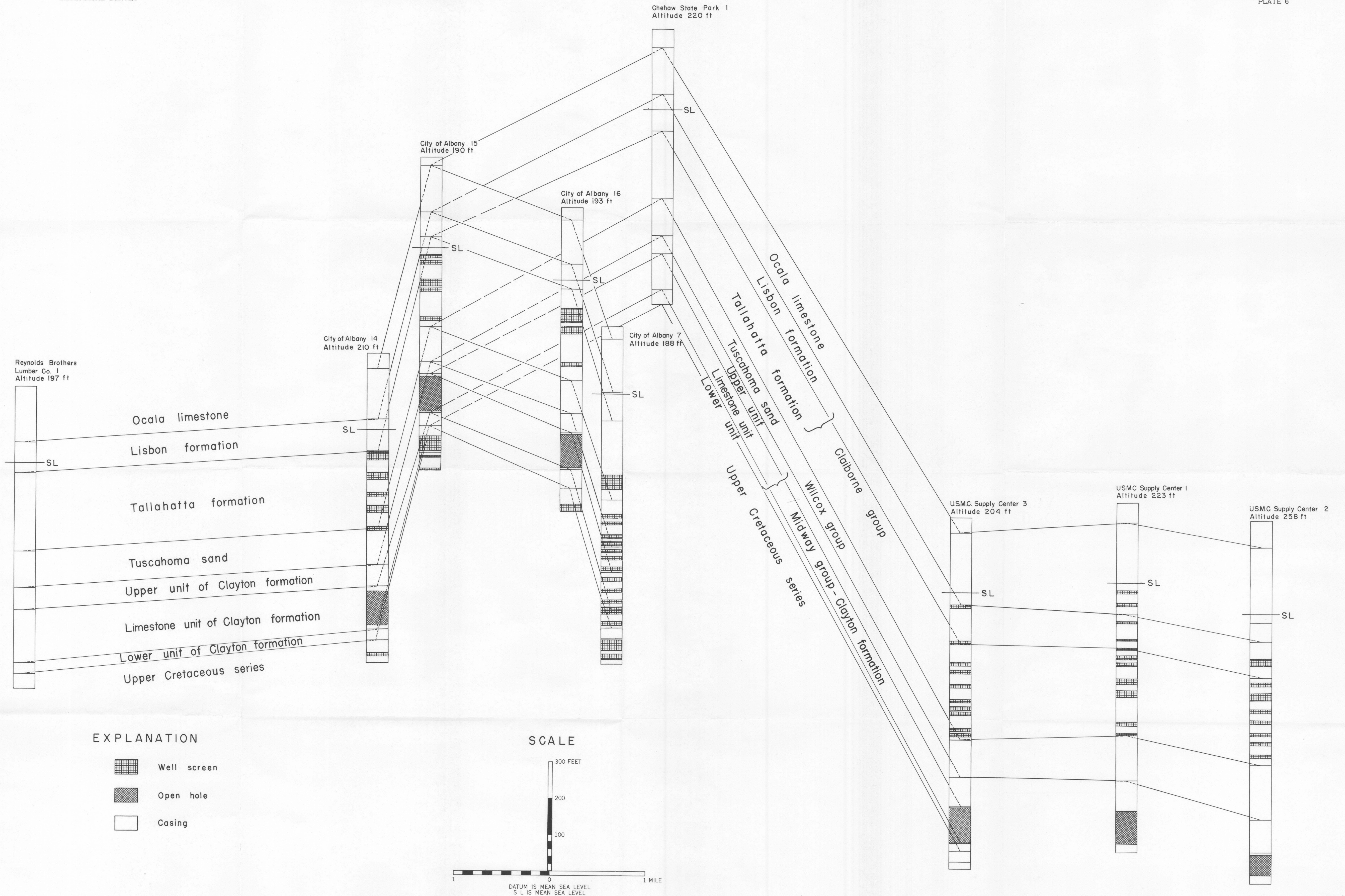
FENCE DIAGRAM SHOWING LOCATION OF WELL SCREENS AND OPEN HOLE IN WELLS OF CITY OF ALBANY AND U. S. MARINE CORPS SUPPLY CENTER, DOUGHERTY COUNTY, GEORGIA
