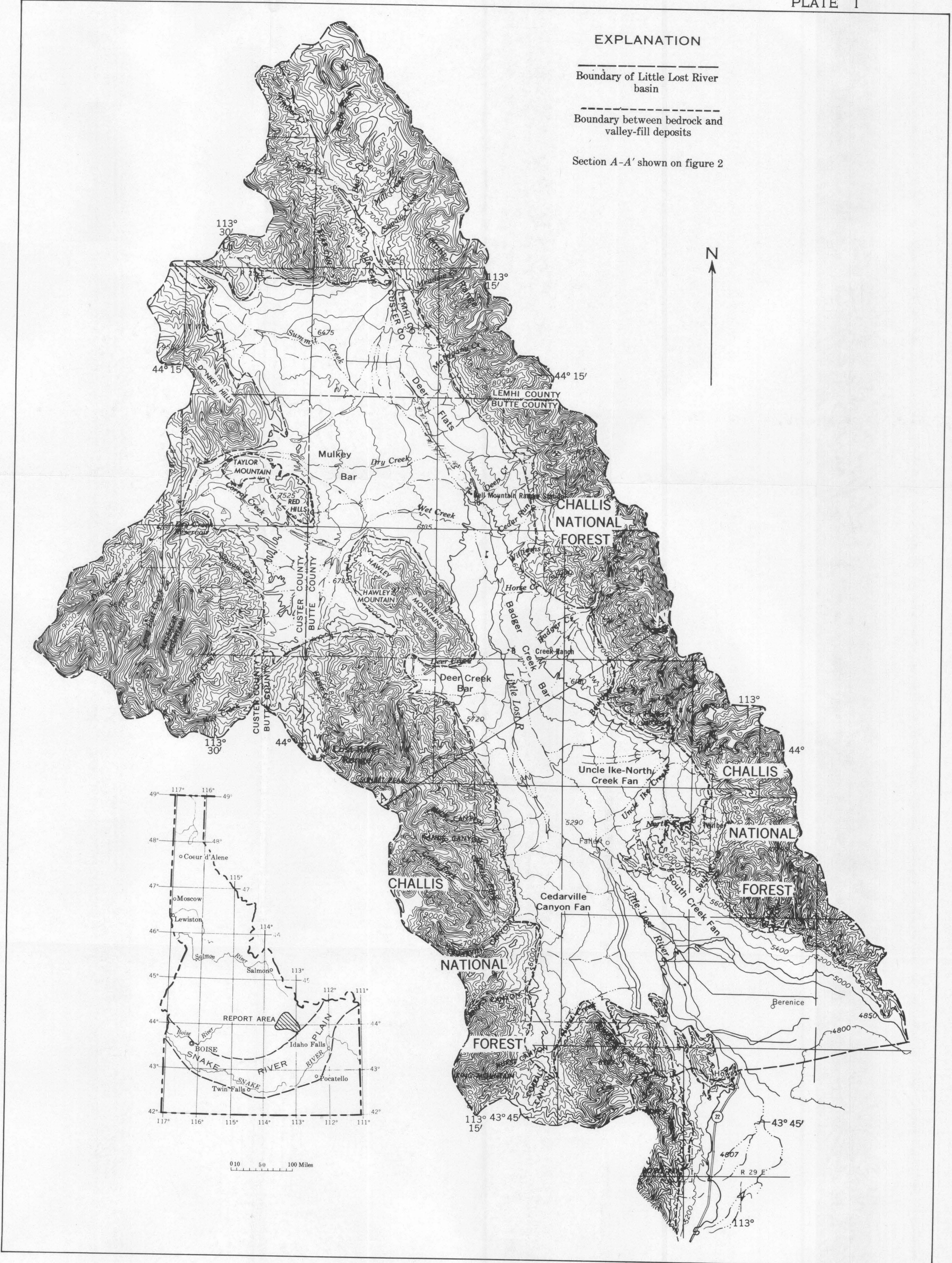
PHYSIOGRAPHIC MAP OF THE LITTLE LOST RIVER BASIN, IDAHO
