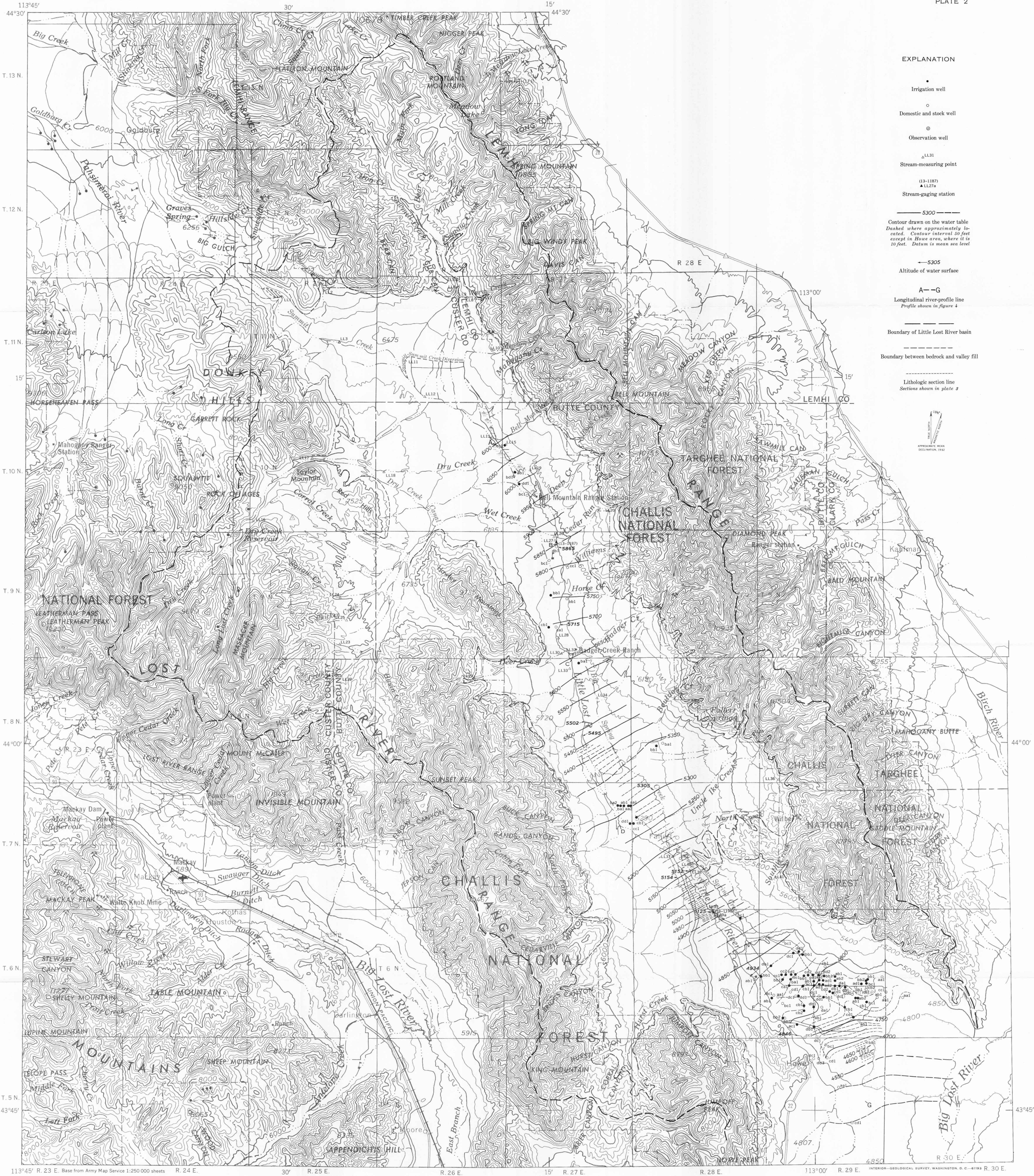
MAP OF THE LITTLE LOST RIVER BASIN, IDAHO, SHOWING SURFACE-AND GROUND-WATER FEATURES
