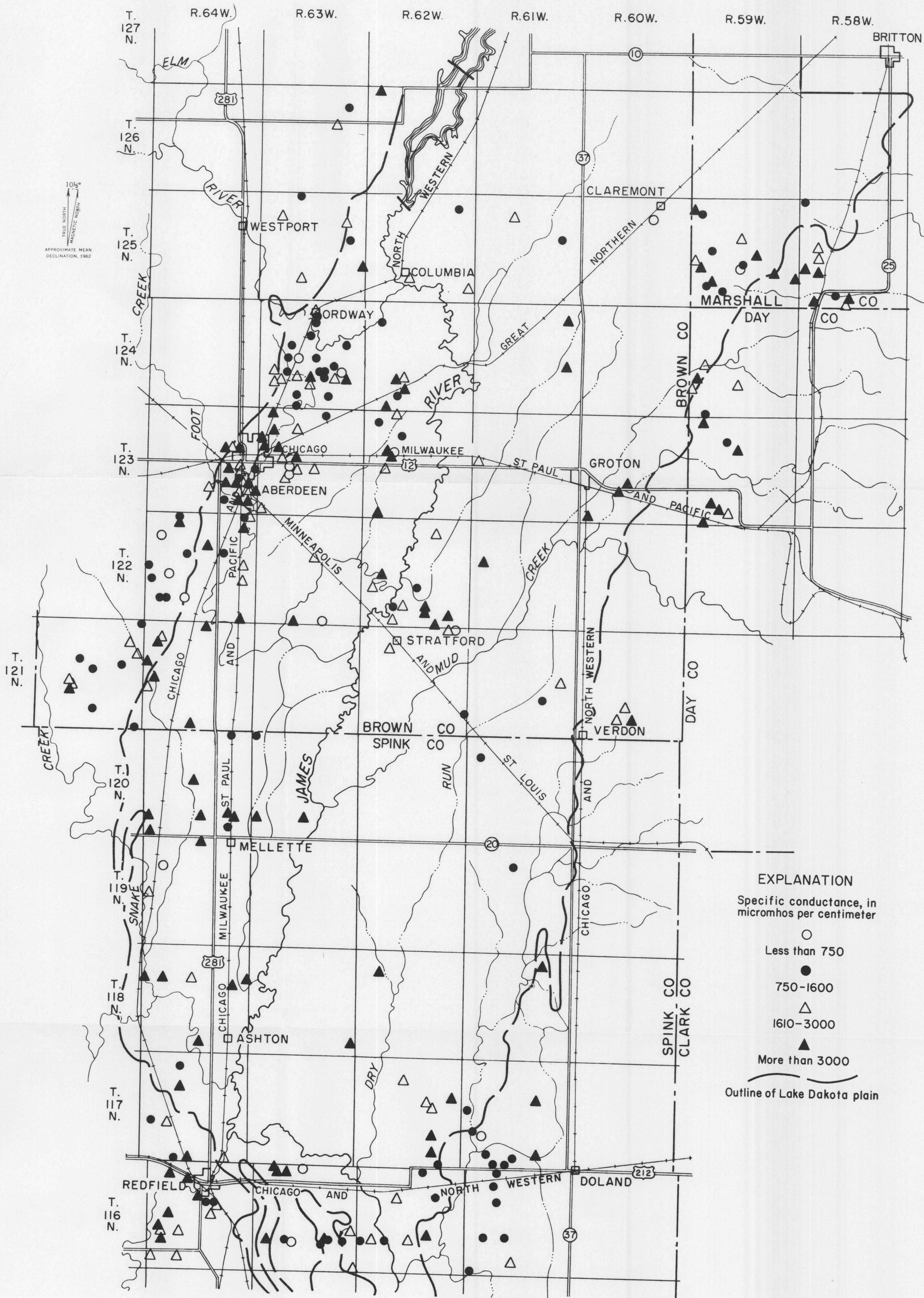
MAP OF THE LAKE DAKOTA PLAIN AREA, SOUTH DAKOTA, SHOWING SPECIFIC CONDUCTANCE OF WATER FROM QUATERNARY DEPOSITS
