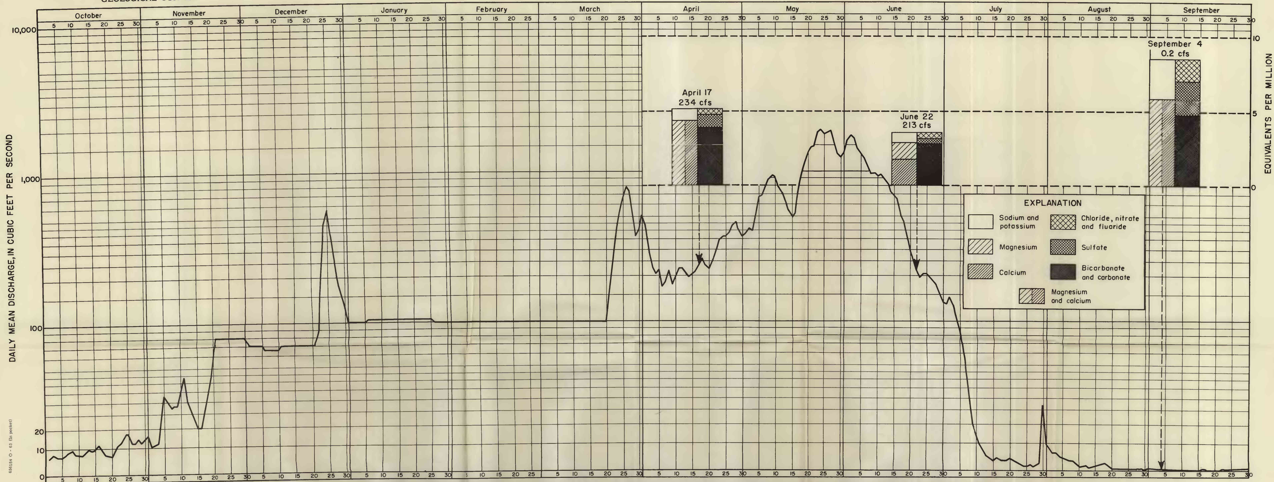
HYDROGRAPH OF BEAR RIVER NORTH OF EVANSTON, WYOMING (16-121-13ba), FROM OCTOBER 1, 1955, TO SEPTEMBER 30, 1956 DIAGRAMS SHOW CHEMICAL COMPOSITION OF WATER IN RELATION TO DISCHARGE. (STREAMFLOWS BELOW 20 CFS ARE RELATIVE AND NOT TO LOG SCALE.)
