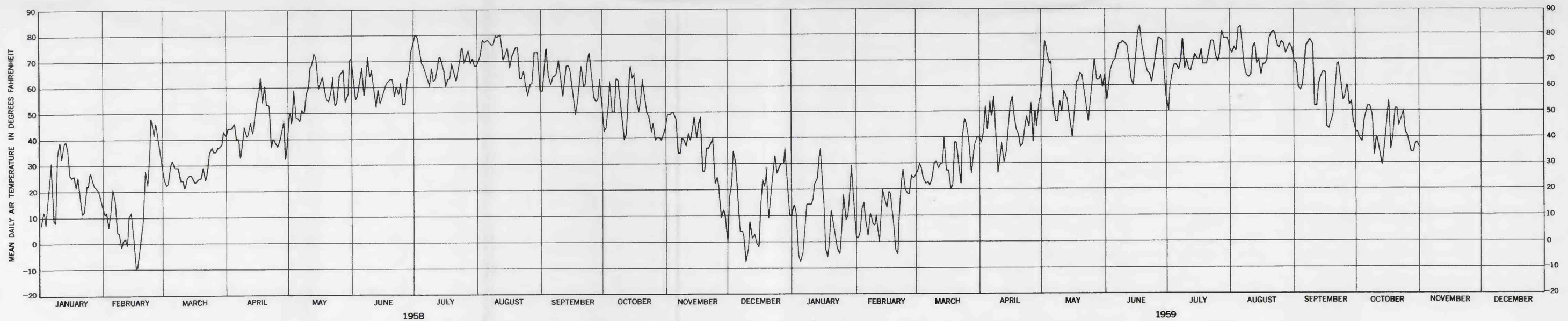
GROUND-WATER THERMOGRAPHS AND GRAPH OF AIR TEMPERATURE AT WORTHINGTON, MINNESOTA
