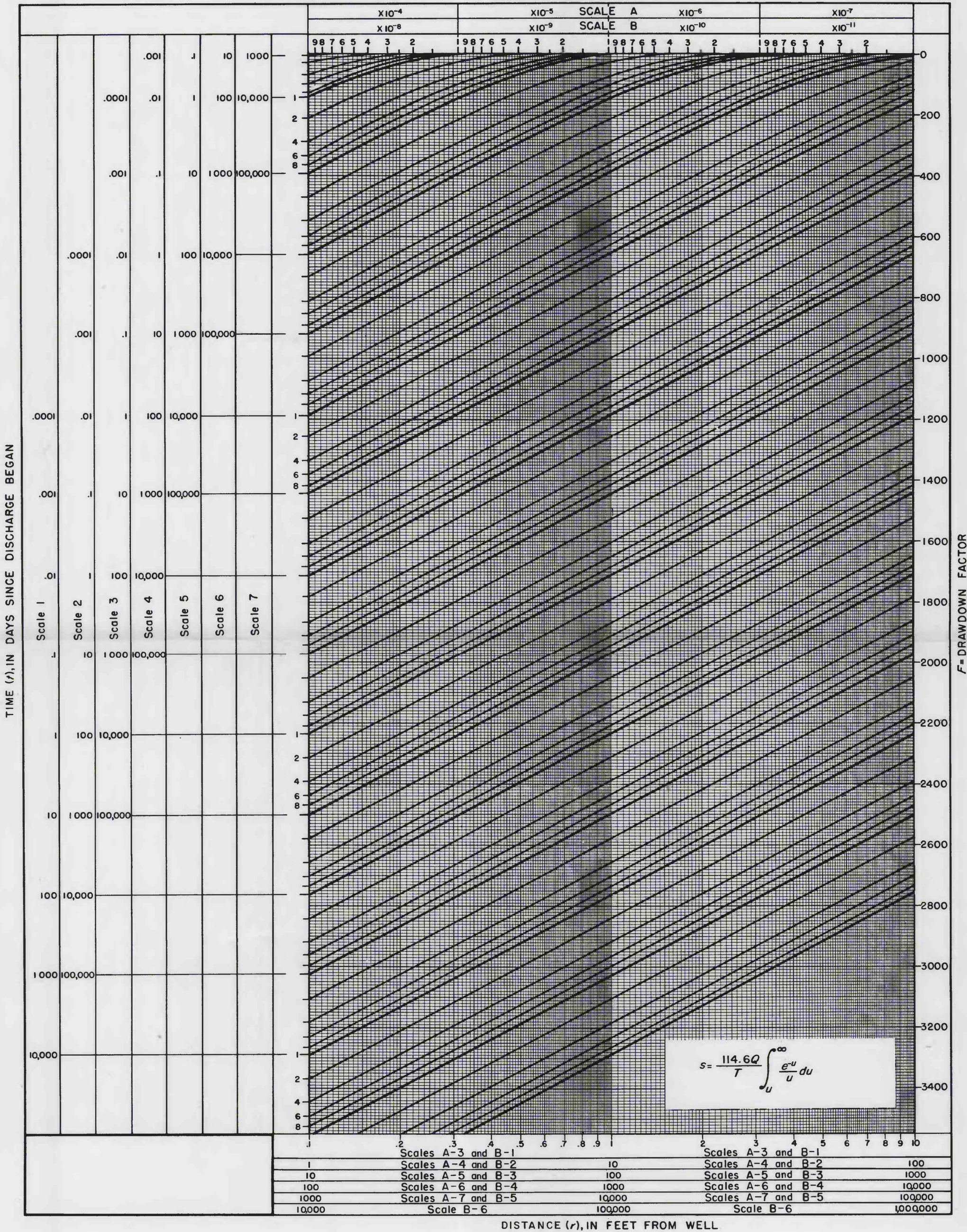
DIAGRAM SHOWING DRAWDOWNS CAUSED BY THE DISCHARGE OF A WELL FROM AN AREALLY EXTENSIVE AQUIFER
