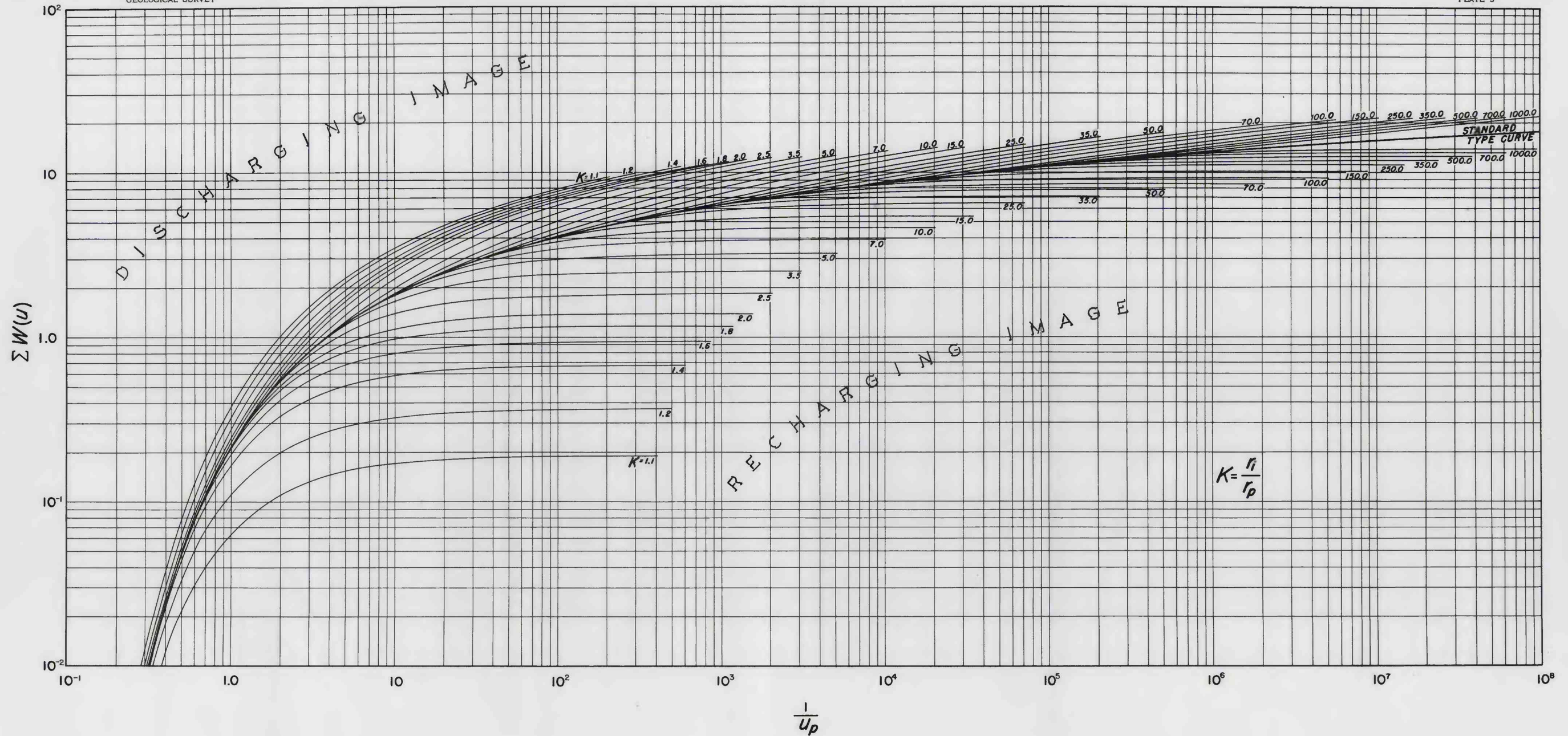
FAMILY OF TYPE CURVES FOR THE SOLUTION OF THE MODIFIED THEIS FORMULA
