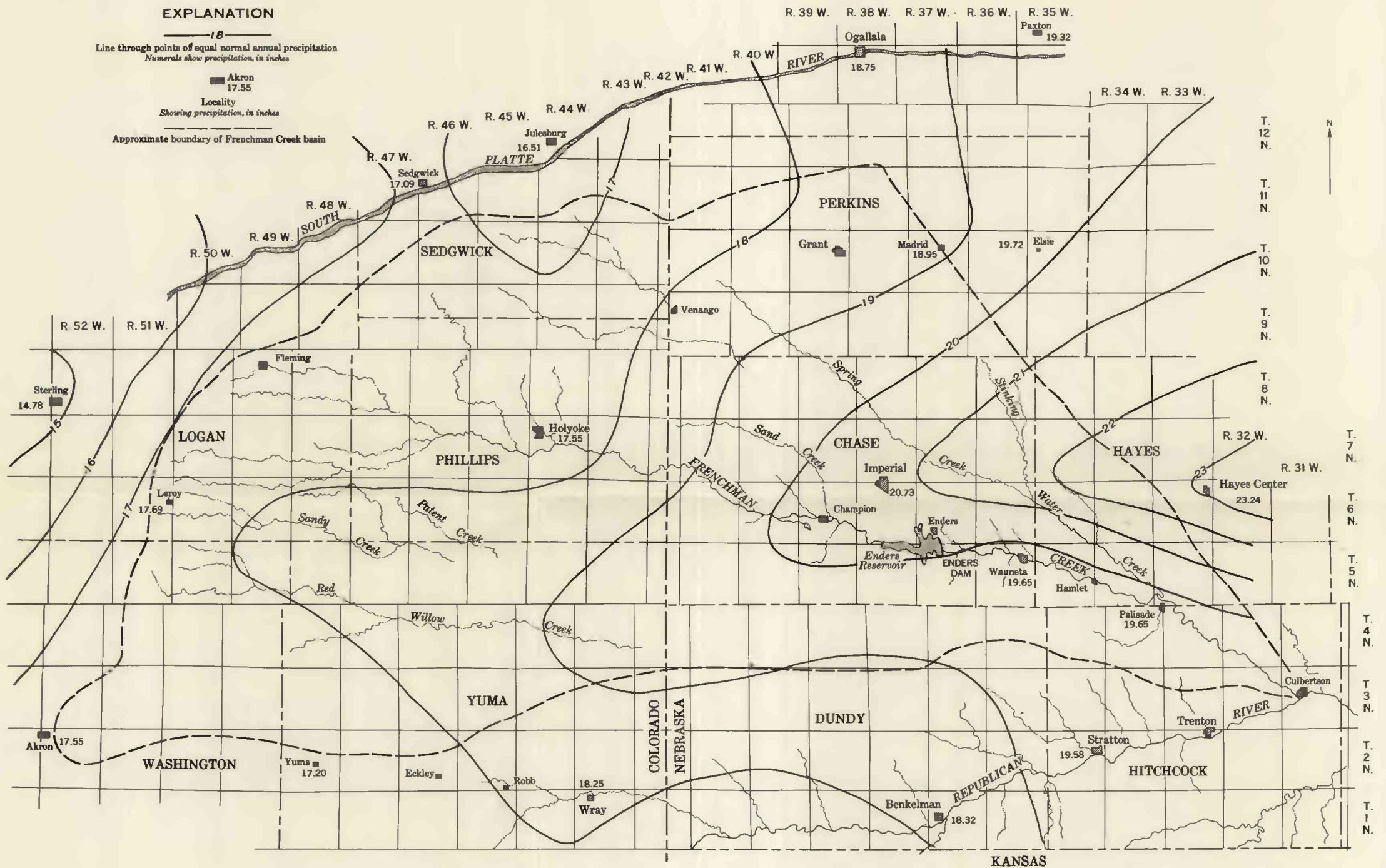
MAP OF FRENCHMAN CREEK BASIN, SHOWING THE DISTRIBUTION OF ANNUAL PRECIPITATION
