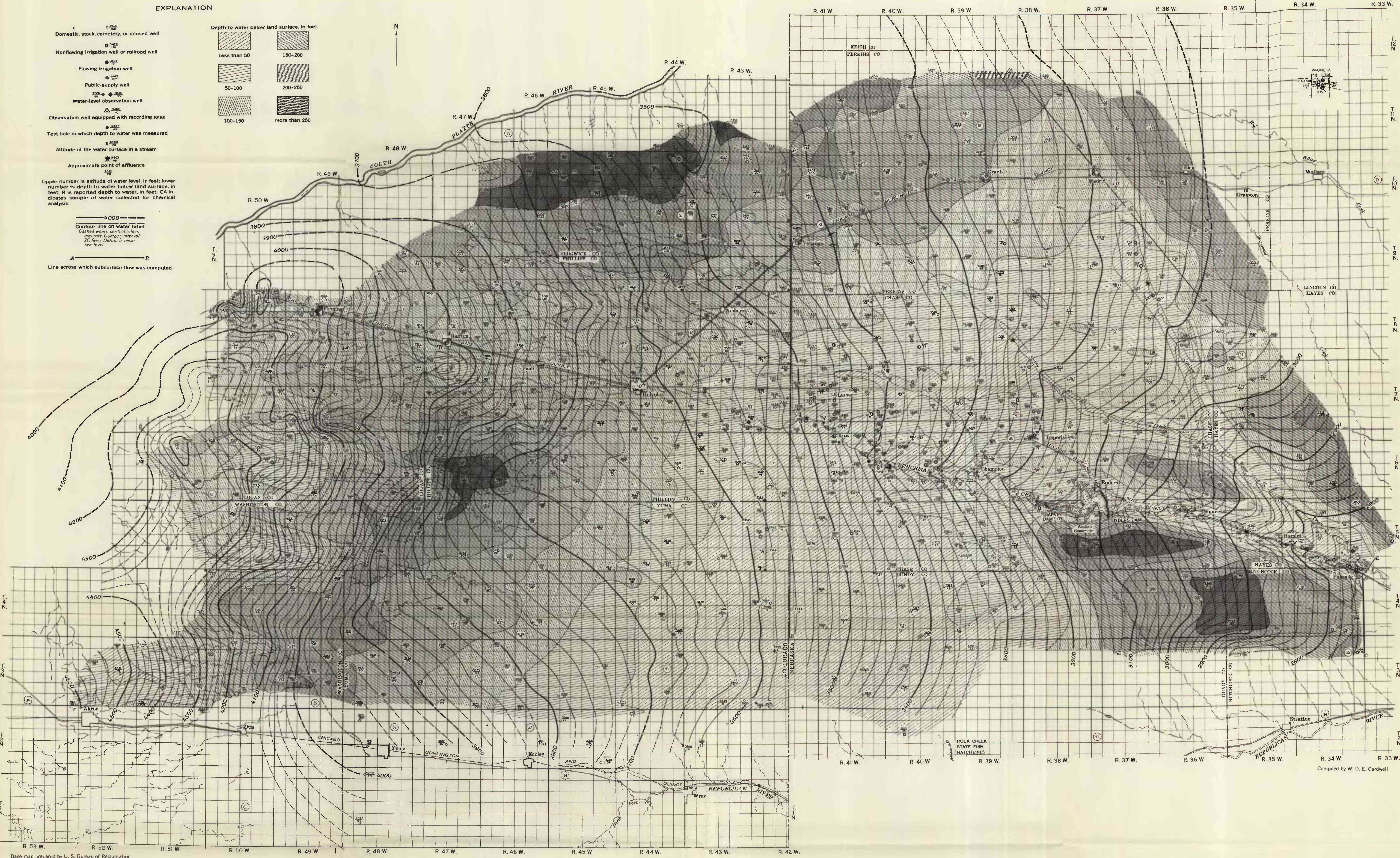
MAP SHOWING LOCATION OF WELLS, DEPTH TO WATER BELOW LAND SURFACE, AND CONFIGURATION OF THE WATER TABLE (SUMMER 1952) IN FRENCHMAN CREEK BASIN
