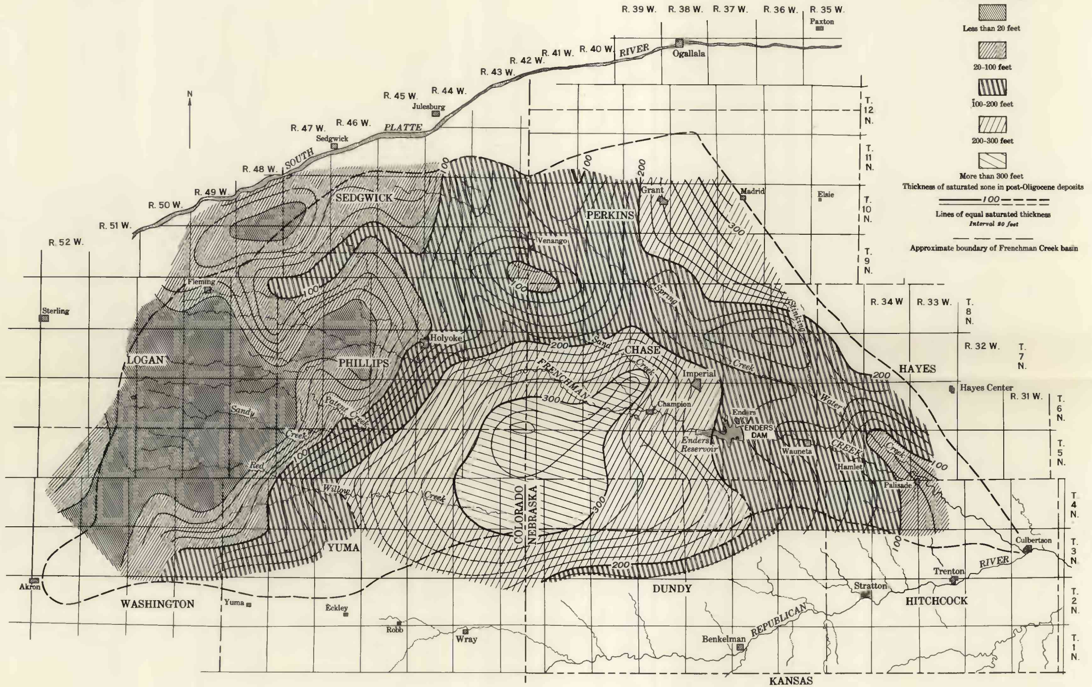
SATURATED THICKNESS OF POST-OLIGOCENE DEPOSITS IN THE FRENCHMAN CREEK BASIN
