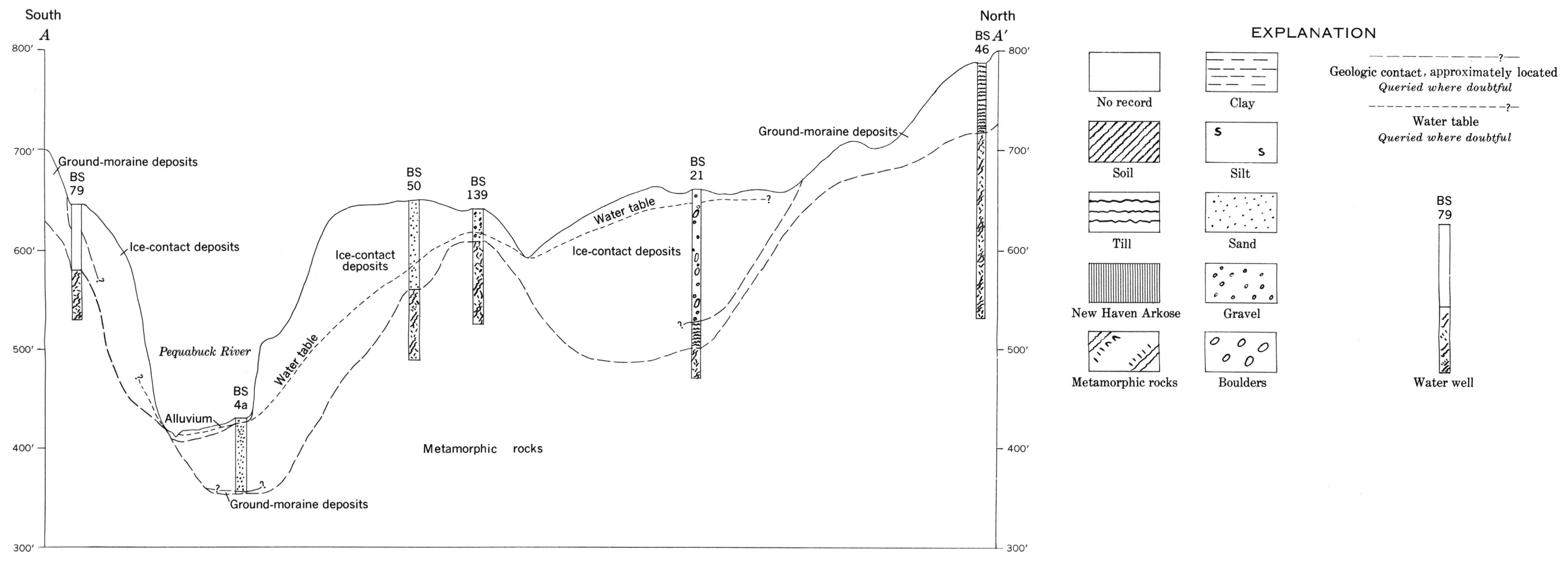
SECTION A-A' ACROSS THE WESTERN UPLAND PART OF THE PEQUABUCK VALLEY
