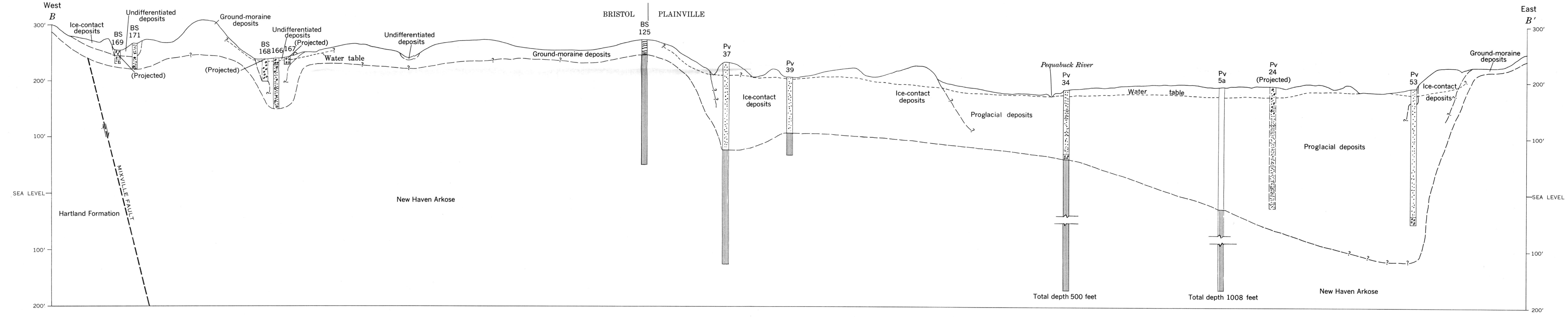
SECTION B-B' ACROSS CENTRAL BRISTOL AND PLAINVILLE
