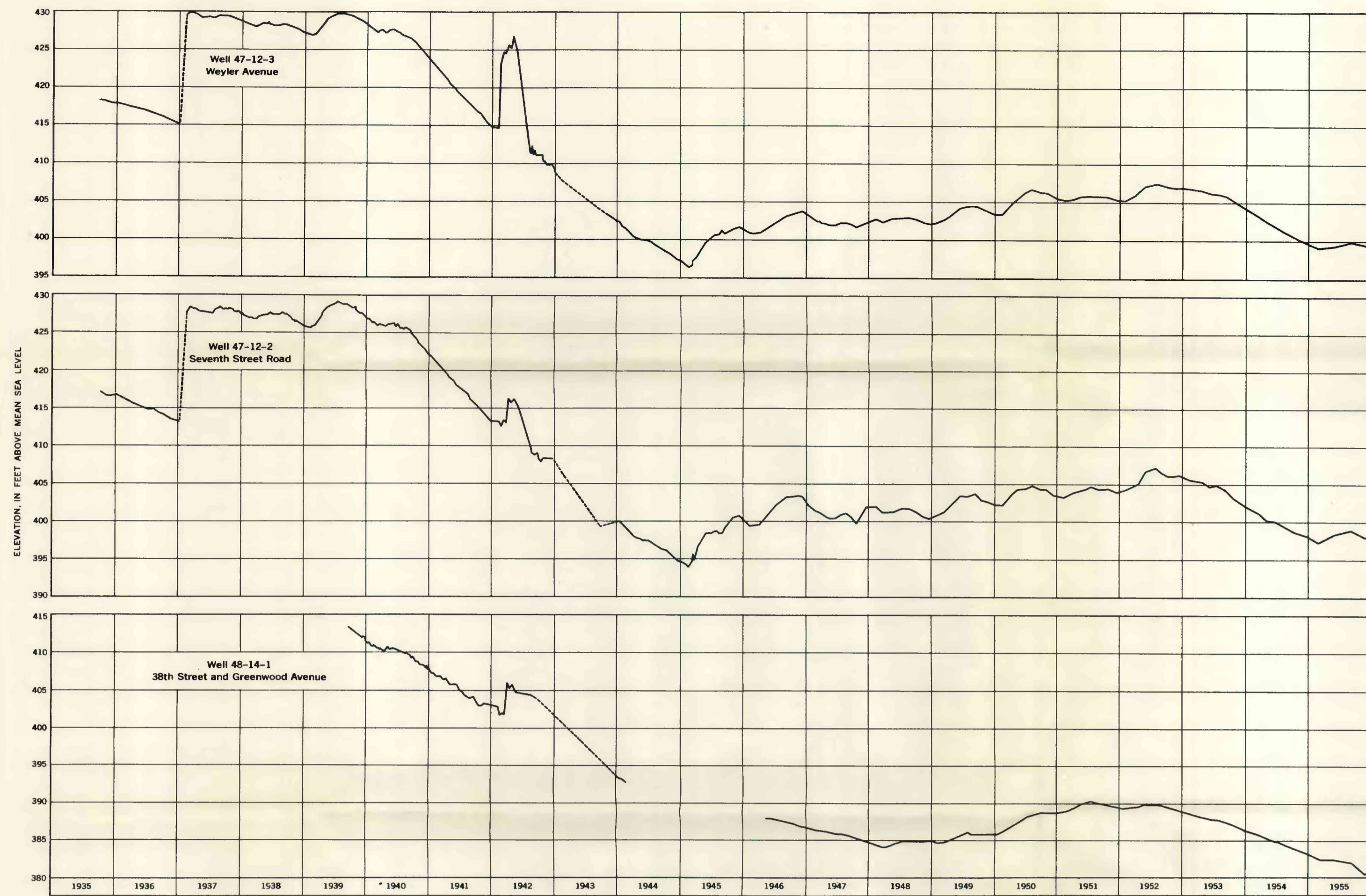
WELLS 47-12-3, 47-12-2, AND 48-14-1
