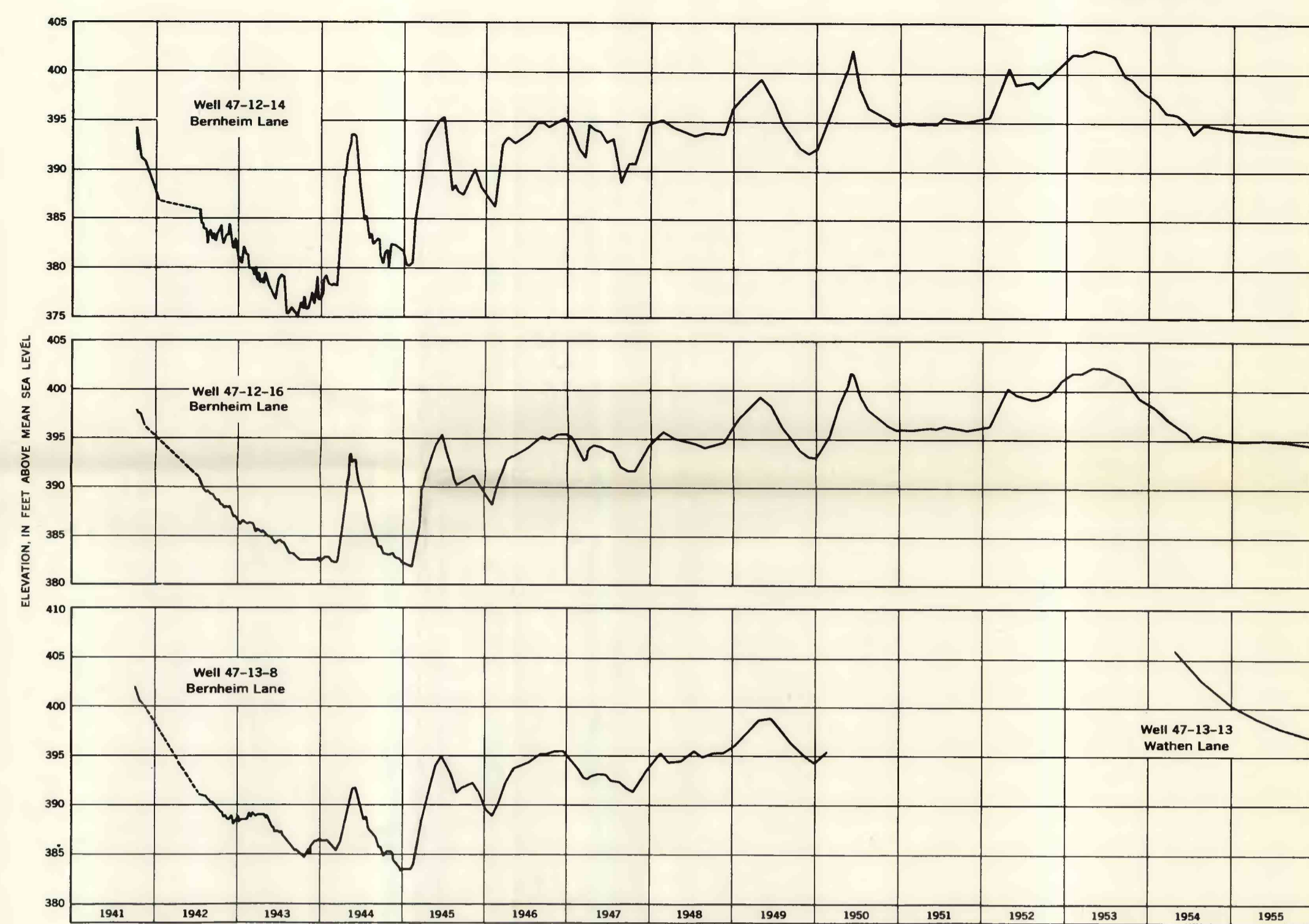
WELLS 47-12-14, 47-12-16, 47-13-8, AND 47-13-13
