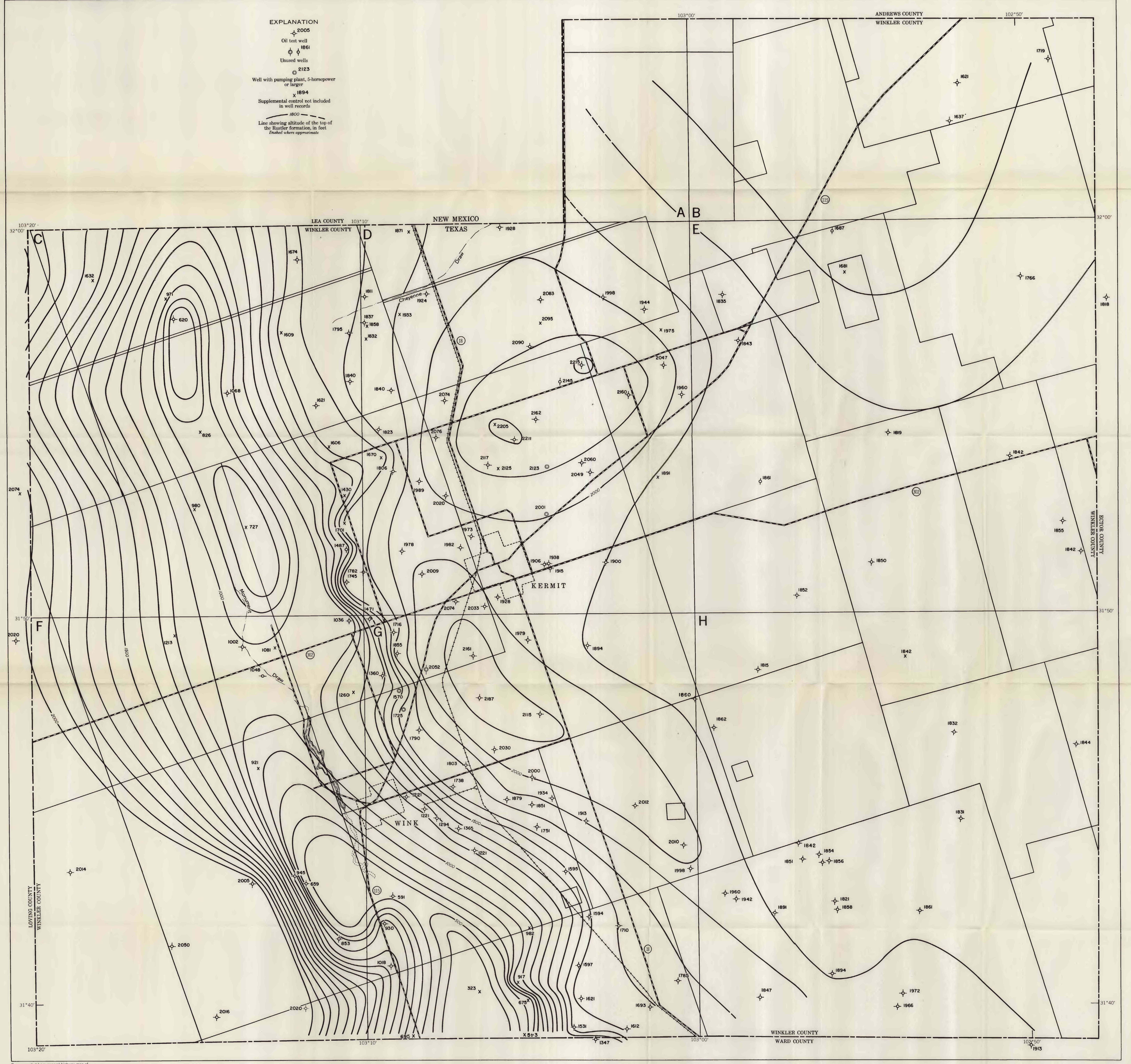
STRUCTURE CONTOUR MAP OF TOP OF RUSTLER FORMATION IN WINKLER COUNTY, TEXAS
