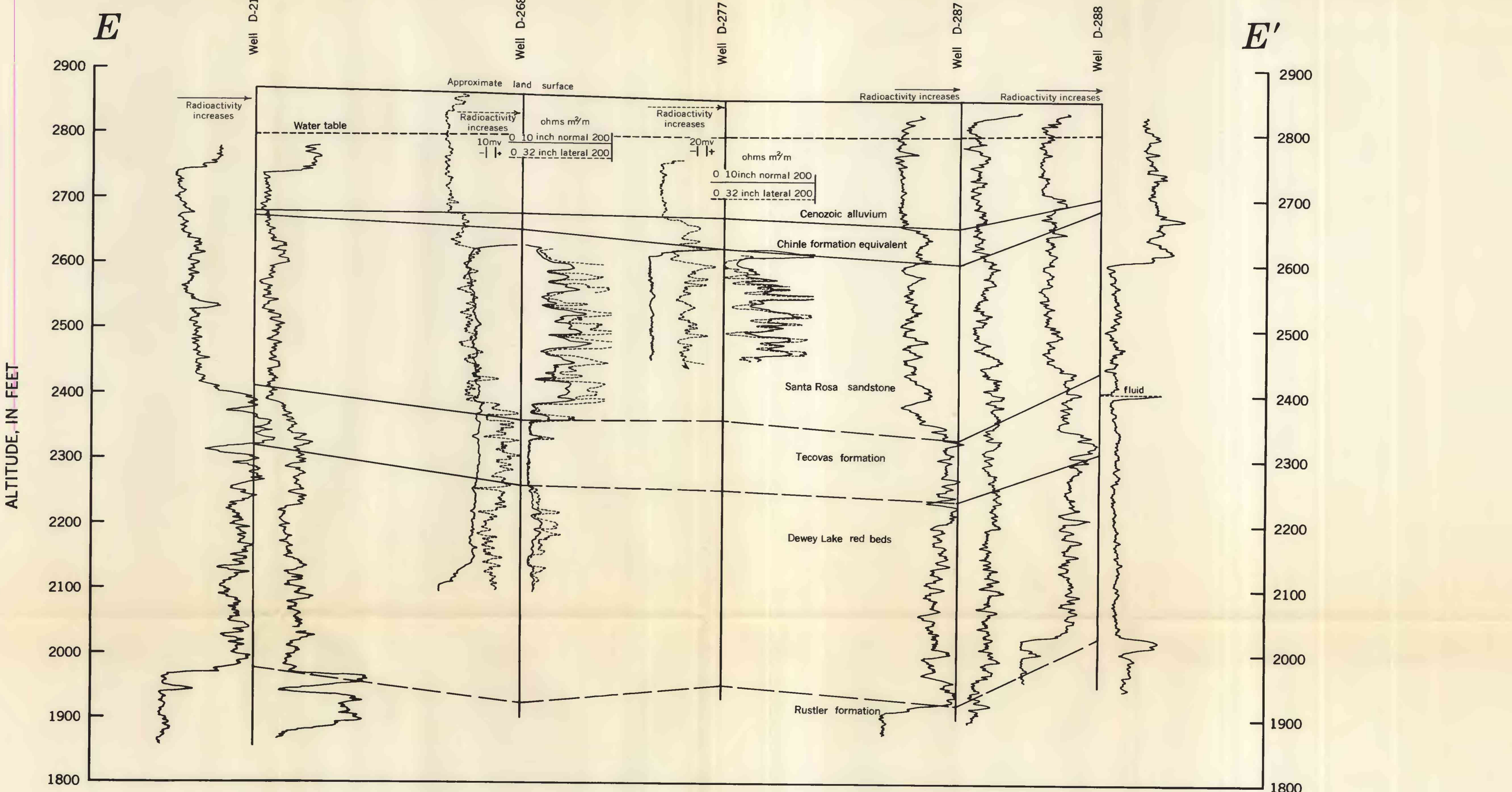
GEOLOGIC CROSS SECTIONS ALONG LINES D-D' AND E-E', VICINITY OF KERMIT, TEXAS
