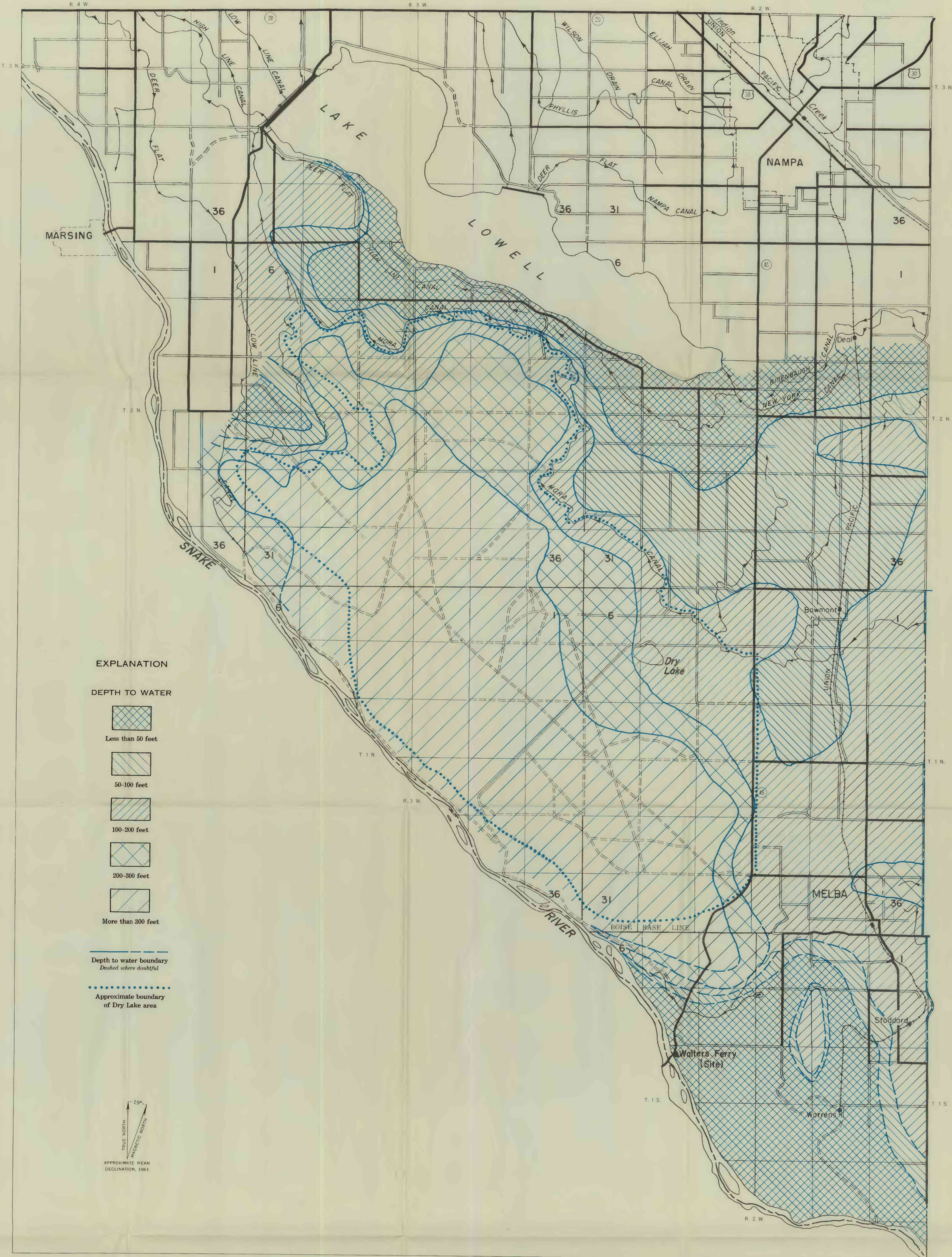
MAP OF SOUTHERN CANYON COUNTY, IDAHO, SHOWING APPROXIMATE DEPTH TO WATER, 1956
