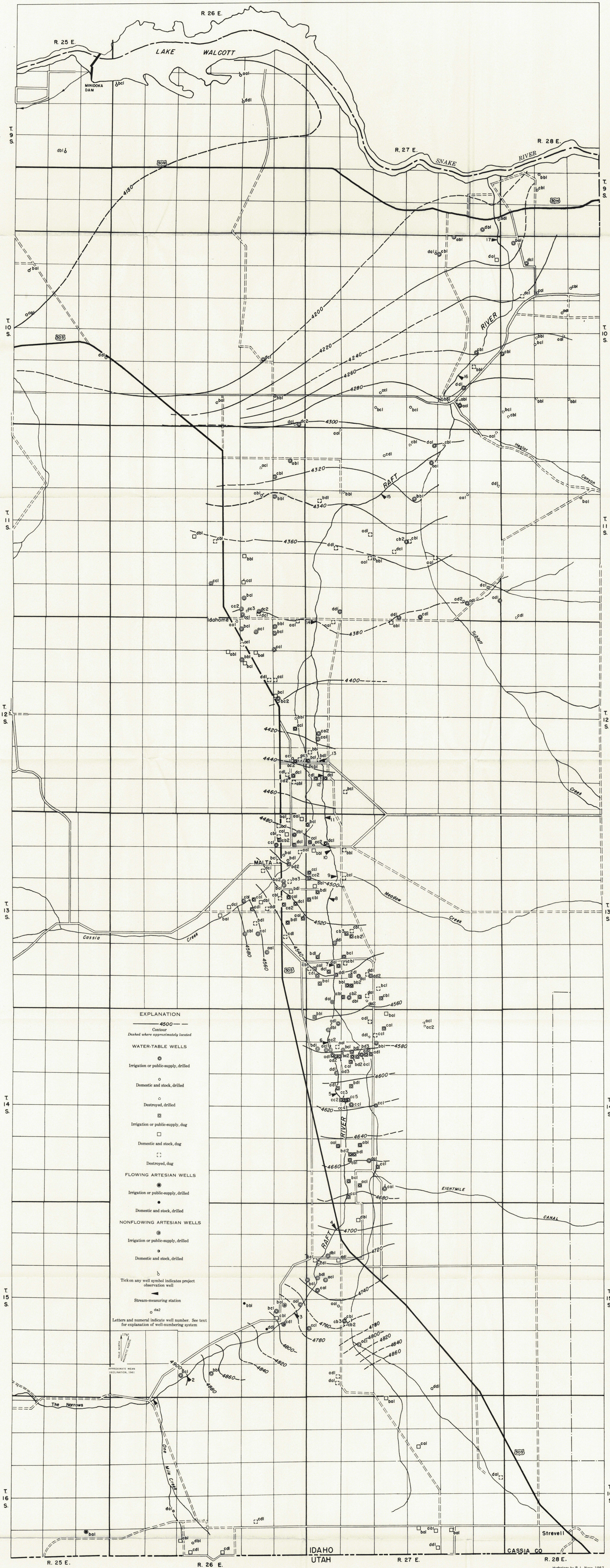
WATER-TABLE CONTOURS IN THE RAFT RIVER VALLEY AND NORTHERN PLAINS SECTION, OCTOBER-NOVEMBER 1952
