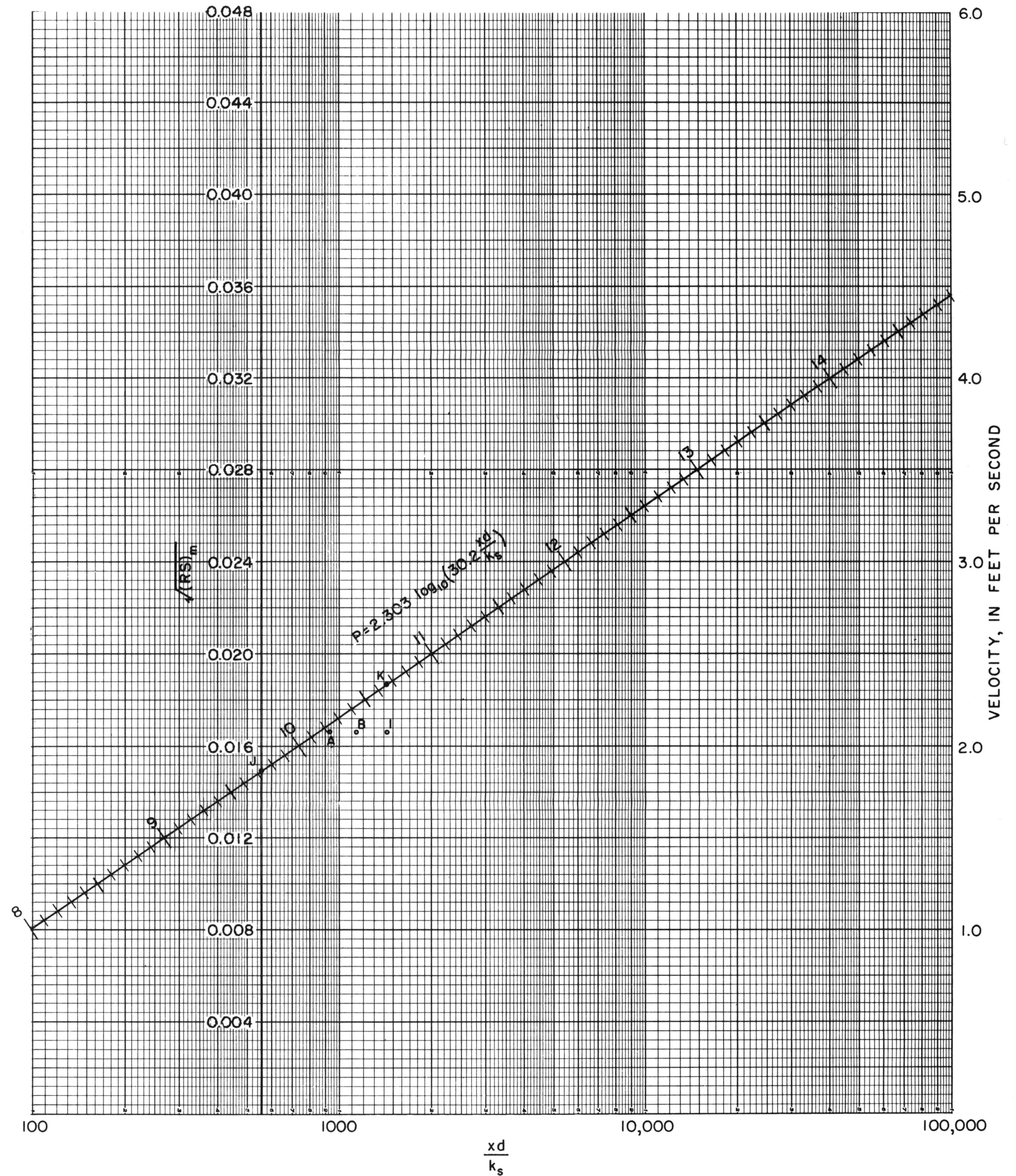
NOMOGRAPH FOR COMPUTING \sqrt{(RS)_m} AND P
