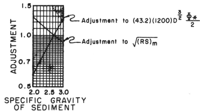
NOMOGRAPH FOR COMPUTING i_B Q_B
