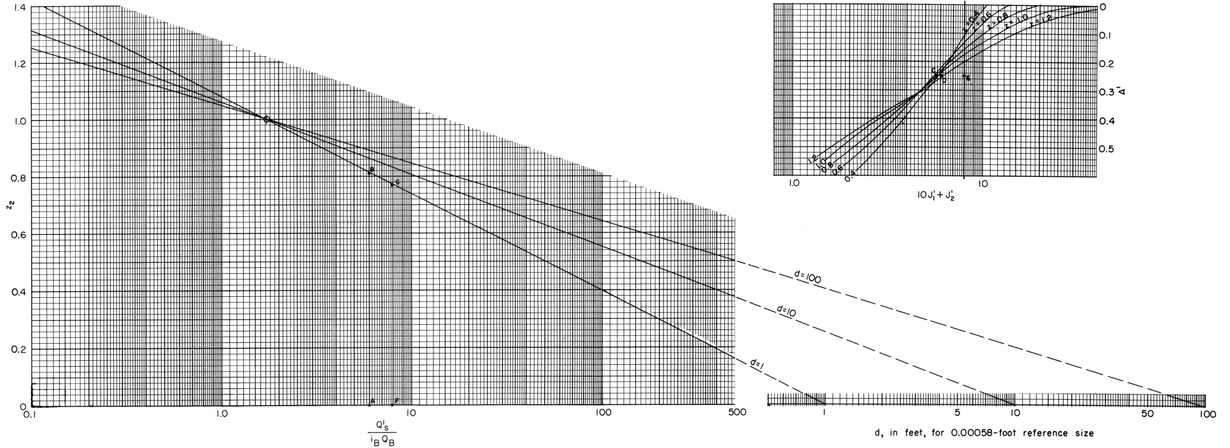
NOMOGRAPH FOR COMPUTING z_2 FROM \frac{Q_s}{i_B Q_B} = \frac{I_1''}{J_1''} (PJ_1' + J_2')
