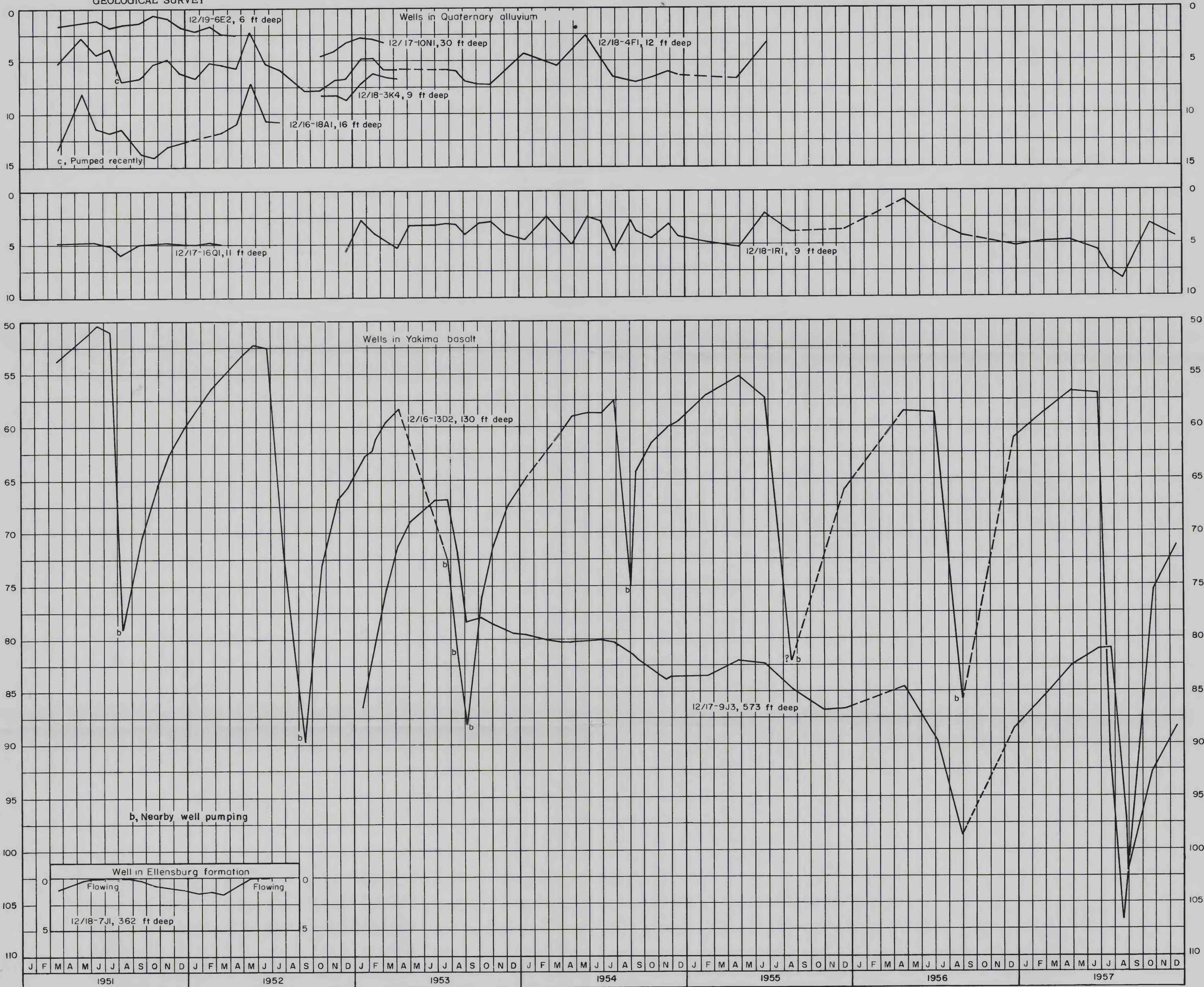
HYDROGRAPHS OF SELECTED WELLS IN AHTANUM VALLEY, YAKIMA COUNTY, WASHINGTON
