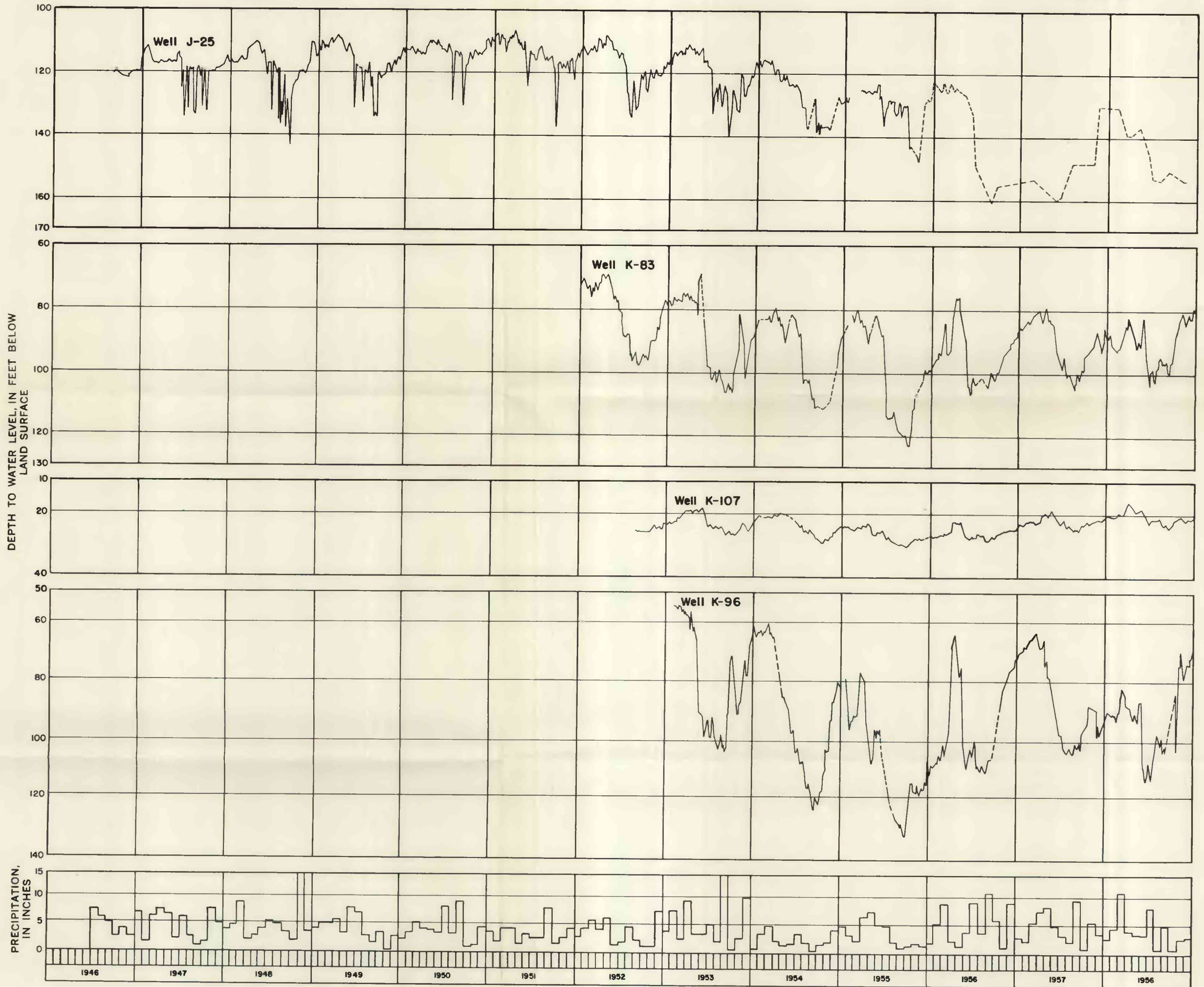
GRAPHS SHOWING CHANGES IN WATER LEVEL IN WELLS J-25, K-83, K-96, AND K-107, AND PRECIPITATION AT MONTGOMERY, ALABAMA
