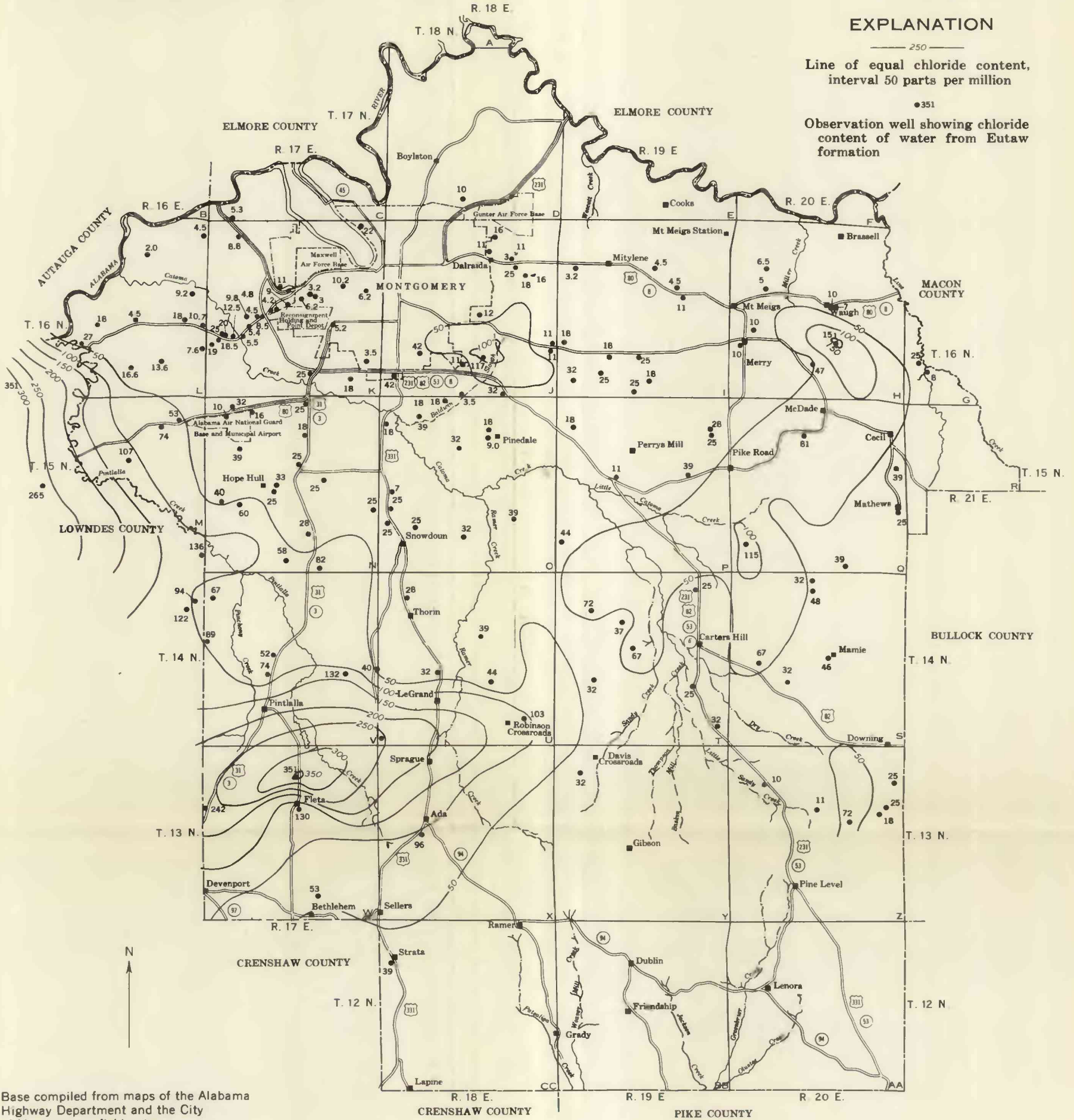
MAP SHOWING CHLORIDE CONTENT OF WATER FROM WELLS IN THE EUTAW FORMATION MONTGOMERY COUNTY, ALABAMA
