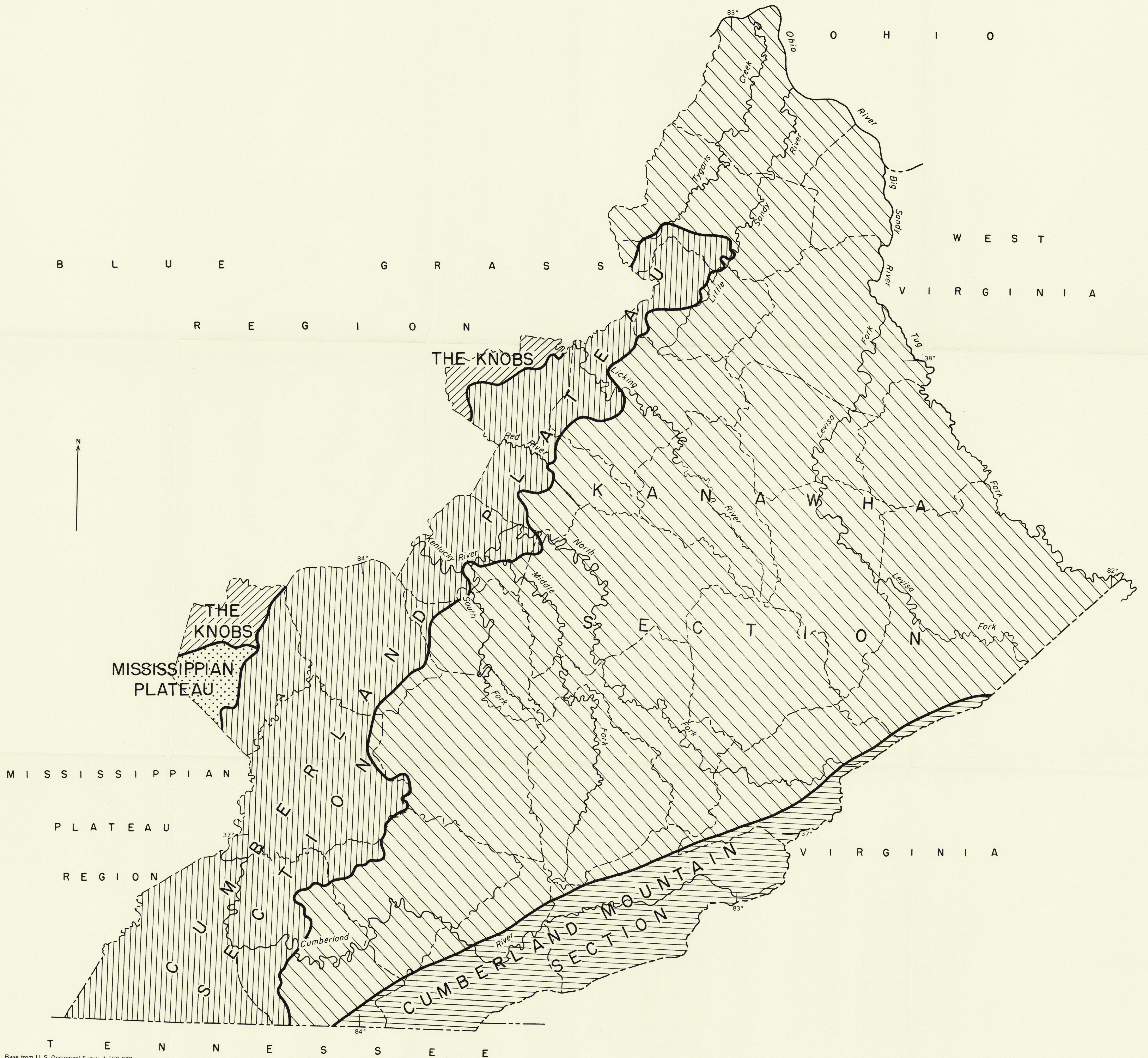
PHYSIOGRAPHIC DIVISIONS OF THE EASTERN COAL FIELD REGION, KENTUCKY
