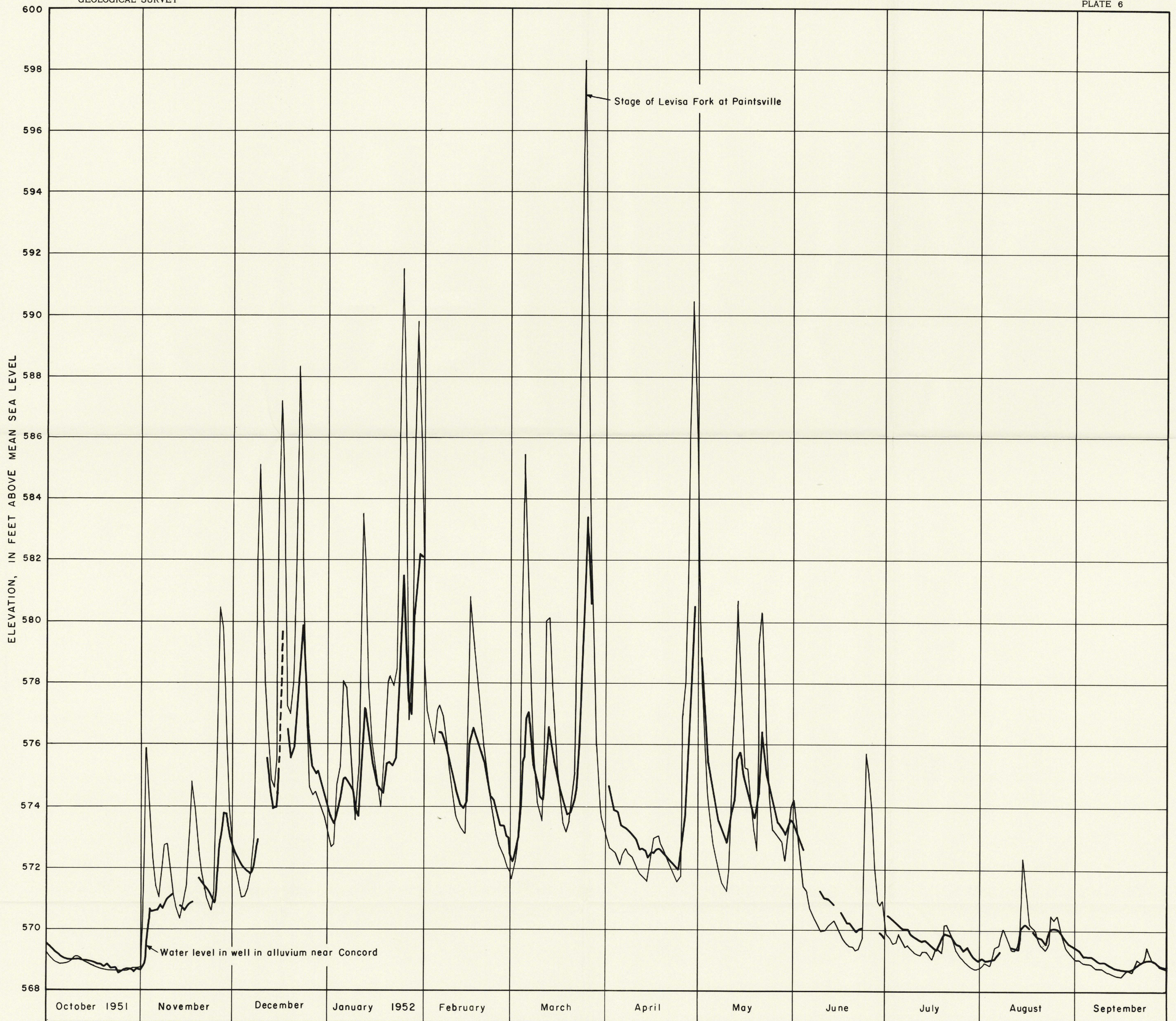
FLUCTUATION OF WATER LEVEL IN A WELL NEAR CONCORD, AND STAGE OF THE LEVISA FORK AT PAINTSVILLE, JOHNSON COUNTY, KENTUCKY
