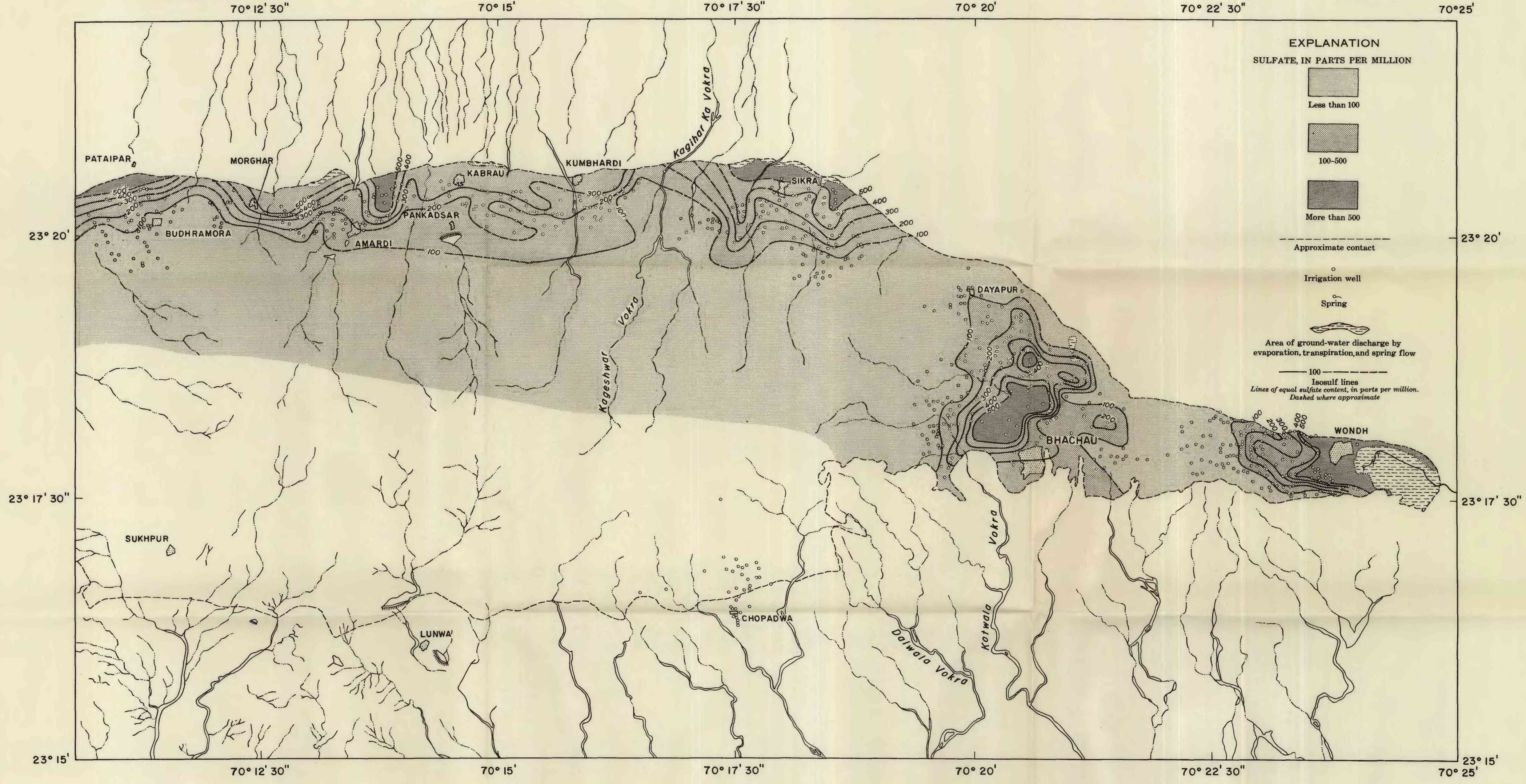
MAP SHOWING AREAL DISTRIBUTION OF SULFATES IN THE SHALLOW GROUND WATER OF THE UPPER BHUJ SERIES IN MARCH-APRIL 1953
