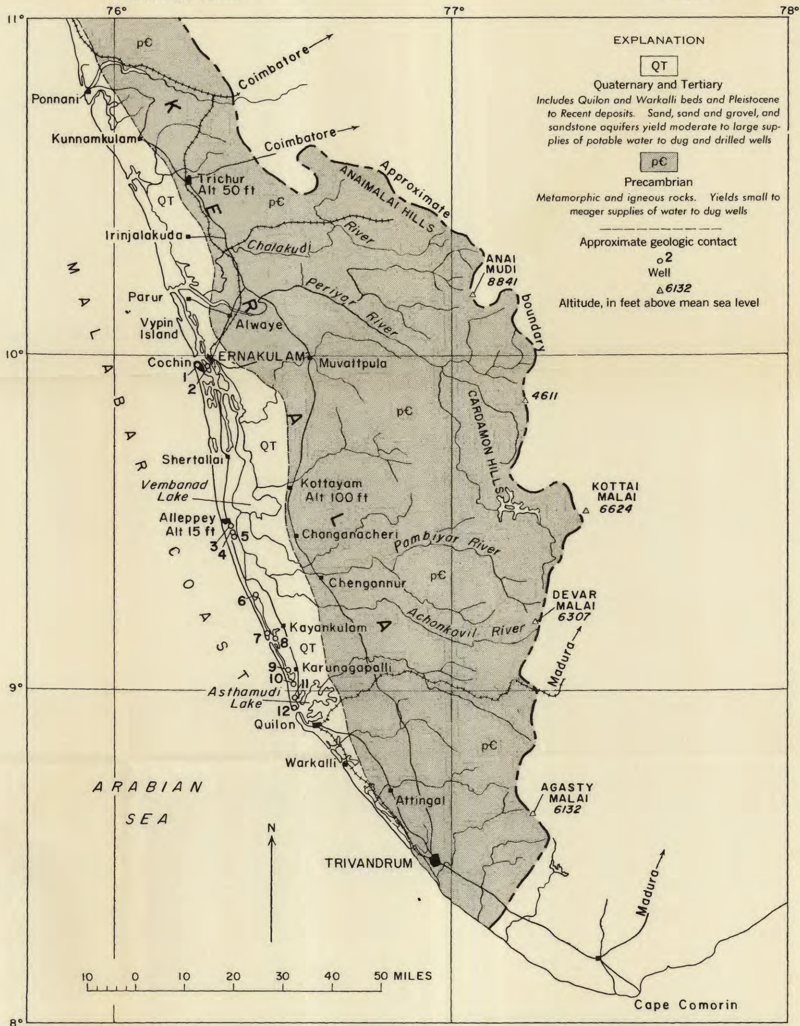
MAP OF SOUTHERN KERALA SHOWING THE LOCATIONS OF TYPICAL WELLS DRILLED IN THE MALABAR COASTAL PLAIN, INDIA
