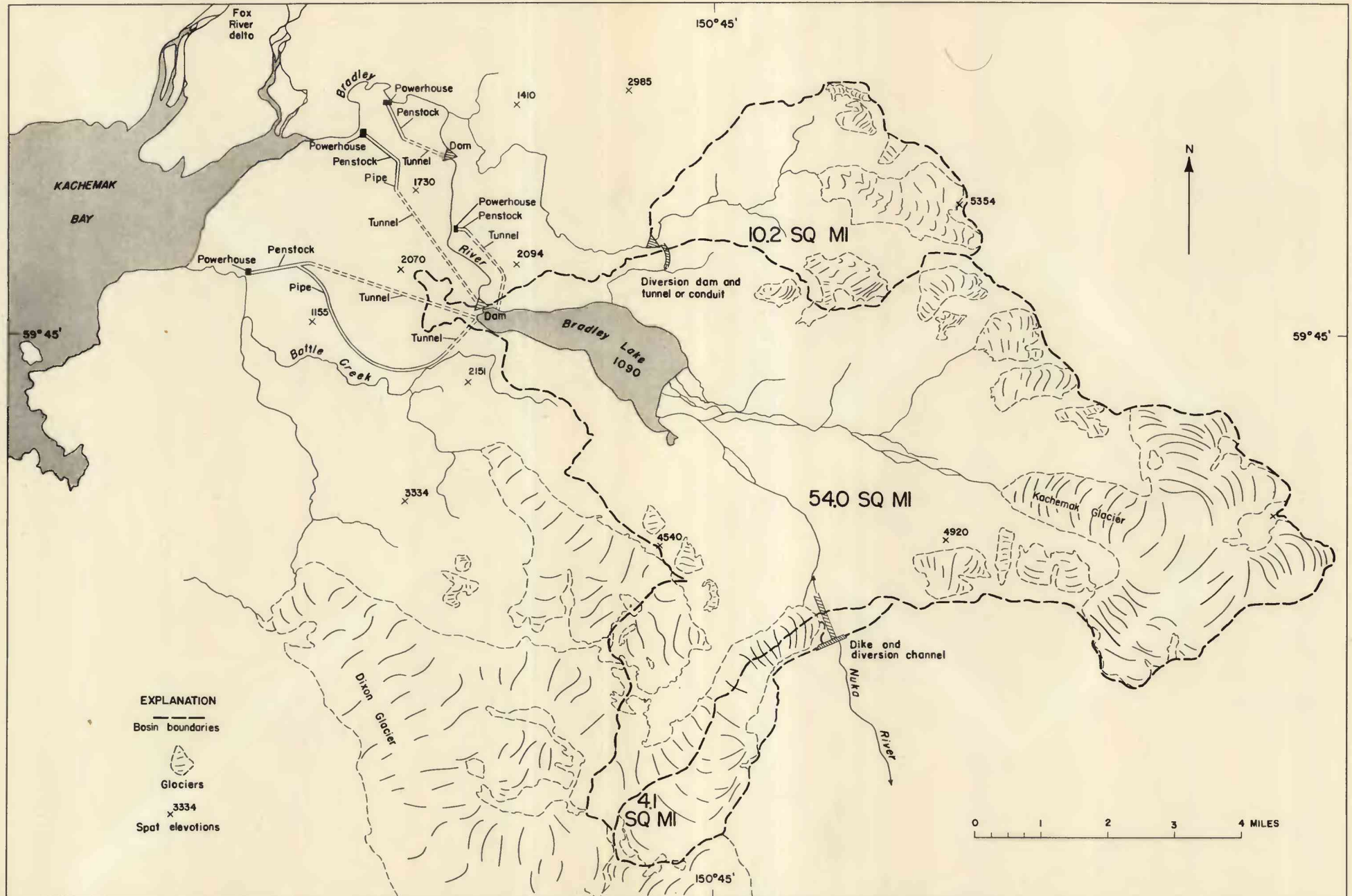
ILLUSTRATIVE PLAN OF WATERPOWER DEVELOPMENT FOR BRADLEY LAKE, ALASKA
