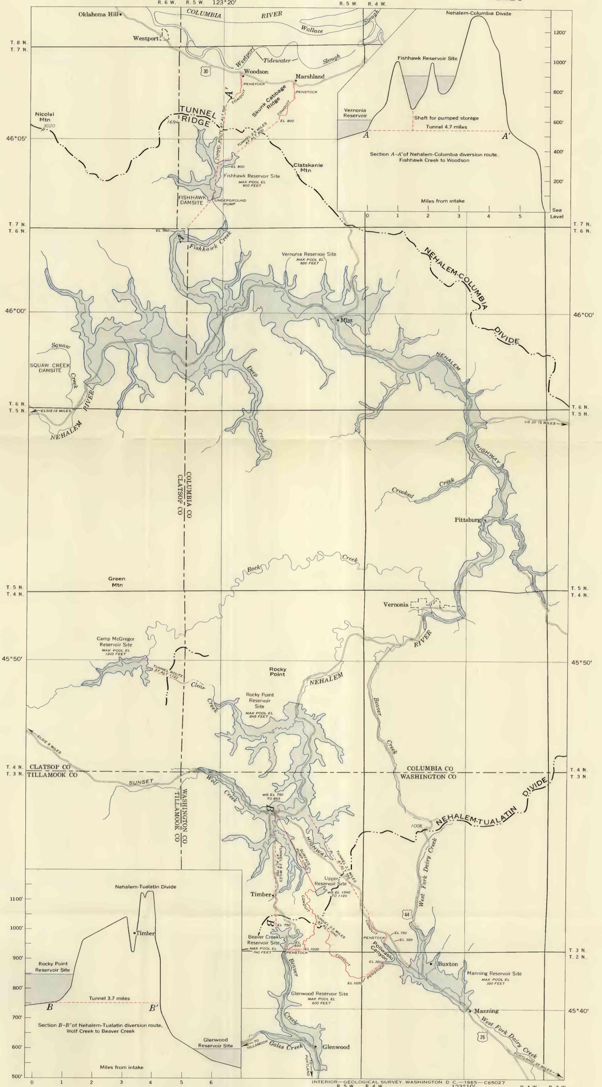
DIVERSION ROUTES AND RELATED STORAGE SITES, NEHALEM-COLUMBIA AND NEHALEM-TUALATIN RIVER BASINS, OREGON
