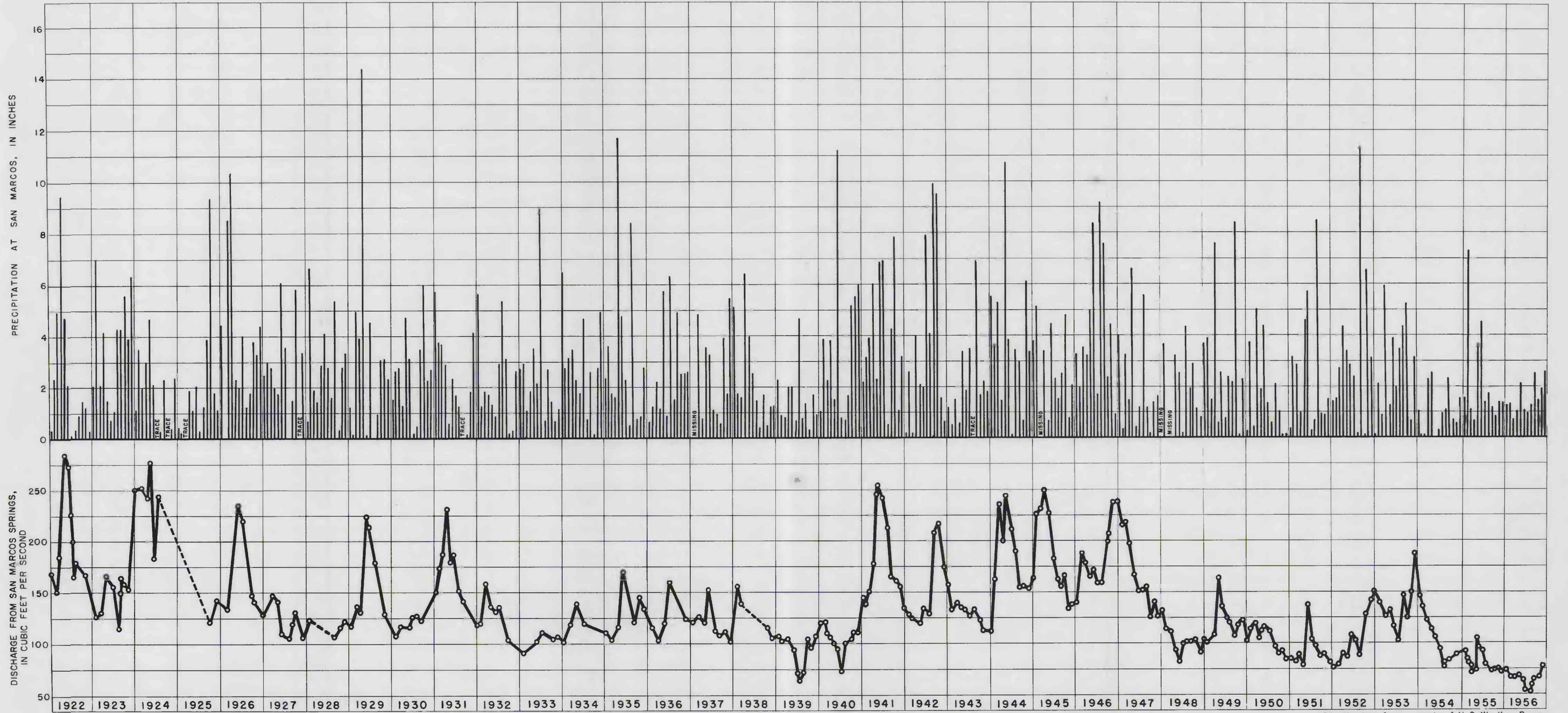
GRAPHS SHOWING MONTHLY PRECIPITATION AT SAN MARCOS AND PERIODICALLY MEASURED DISCHARGE OF SAN MARCOS SPRINGS, TEXAS, 1922-56
