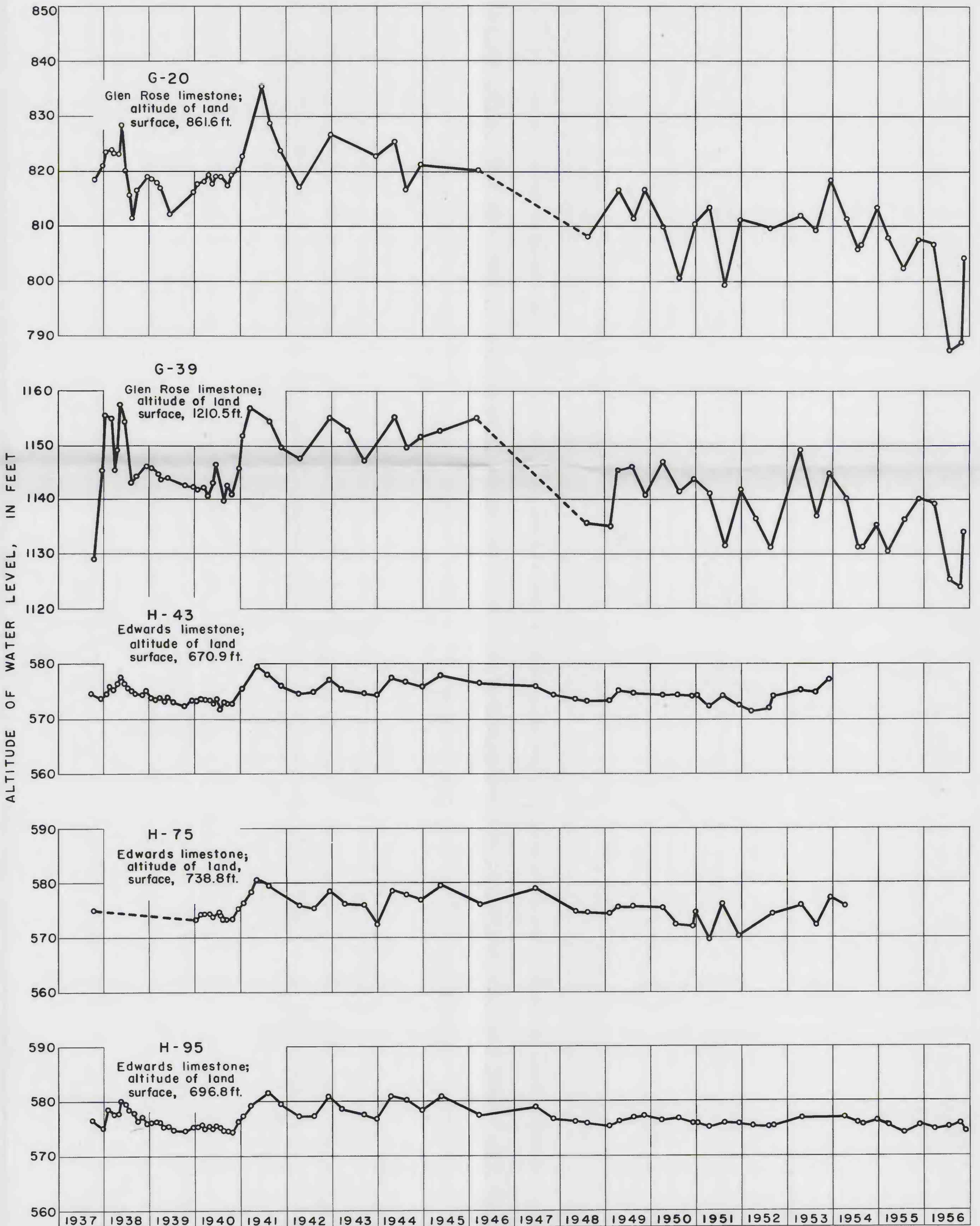
HYDROGRAPHS OF 2 WELLS IN THE GLEN ROSE LIMESTONE NEAR WIMBERLEY AND 3 WELLS IN THE EDWARDS LIMESTONE NEAR SAN MARCOS, TEXAS, 1937-56
