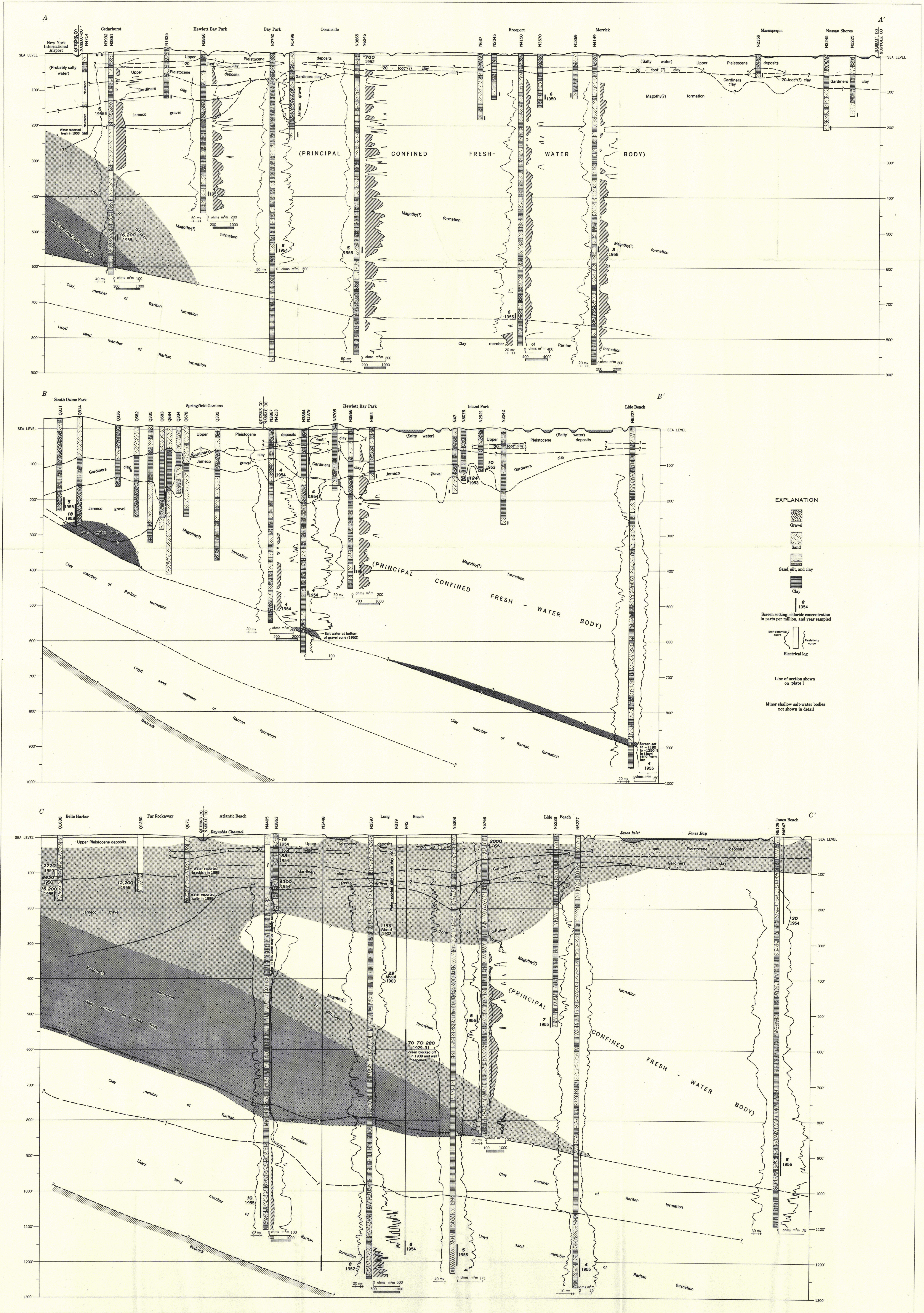
GEOLOGIC SECTIONS A-A', B-B', AND C-C' OF SOUTHERN NASSAU AND SOUTHEASTERN QUEENS COUNTIES LONG ISLAND, NEW YORK
