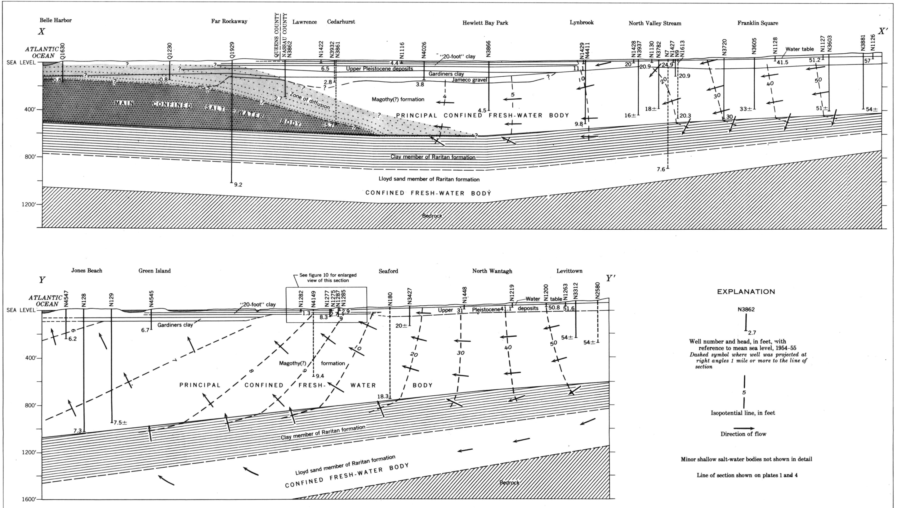
SECTIONS X-X' AND Y-Y' SHOWING PROBABLE FLOW OF WATER IN PRINCIPAL ARTESIAN AQUIFER IN SOUTHWESTERN AND SOUTHEASTERN NASSAU COUNTY, NEW YORK
