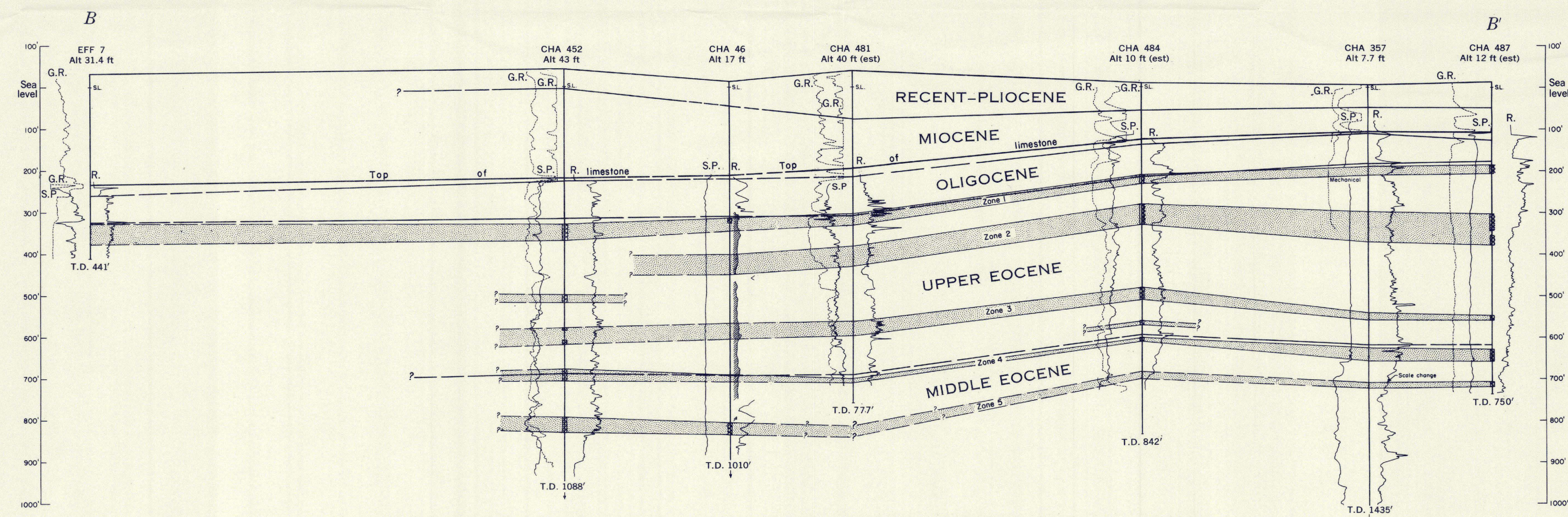
GEOLOGIC SECTIONS A-A' AND B-B' SHOWING WATER-YIELDING ZONES IN PRINCIPAL ARTESIAN AQUIFER OF SAVANNAH AREA
