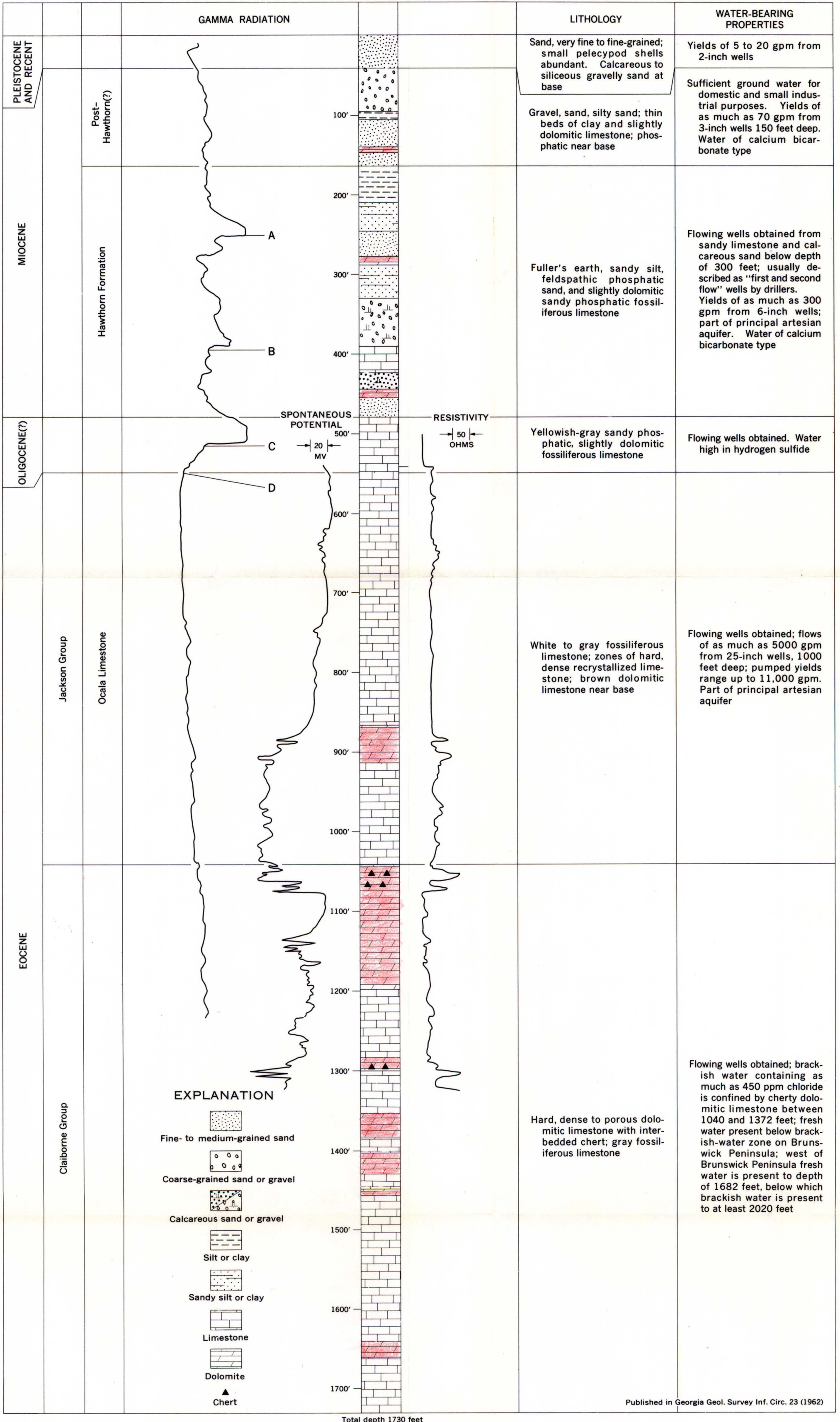
GENERALIZED GEOLOGIC SECTION OF GLYNN COUNTY, GEORGIA, AS DETERMINED FROM TEST WELL 2 (D-182), AND WATER-BEARING PROPERTIES OF THE ROCKS
