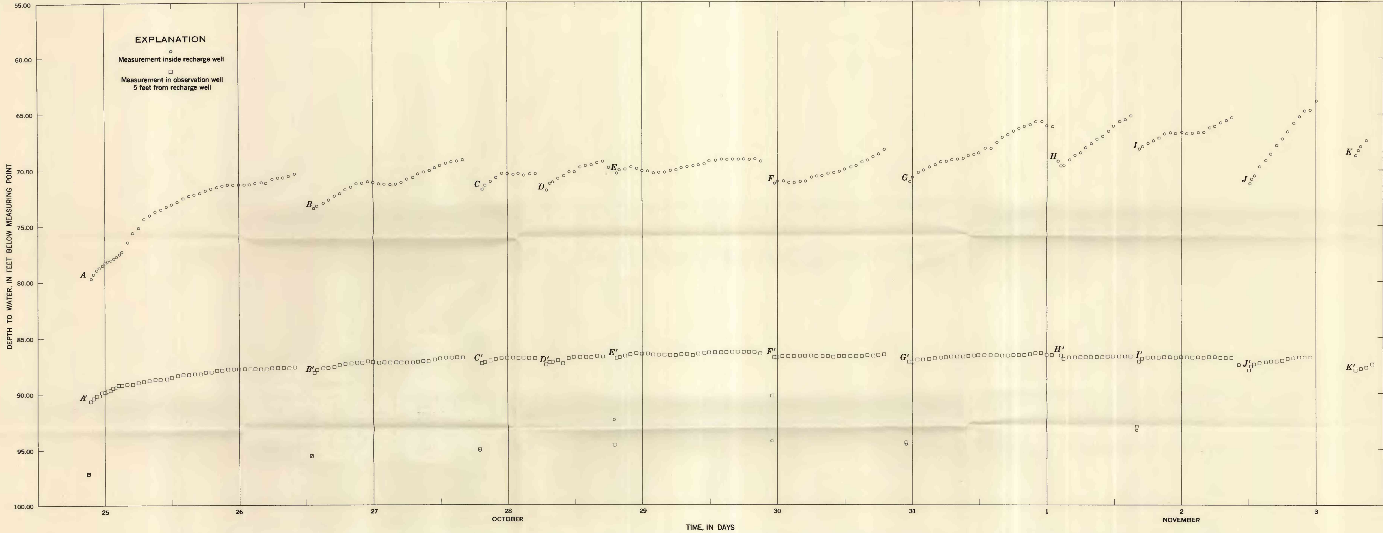
ARITHMETIC PLOTS OF THE WATER LEVELS INSIDE THE RECHARGE WELL AND IN AN OBSERVATION WELL 5 FEET FROM THE RECHARGE WELL DURING TEST 13, GRAND PRAIRIE REGION, ARKANSAS
