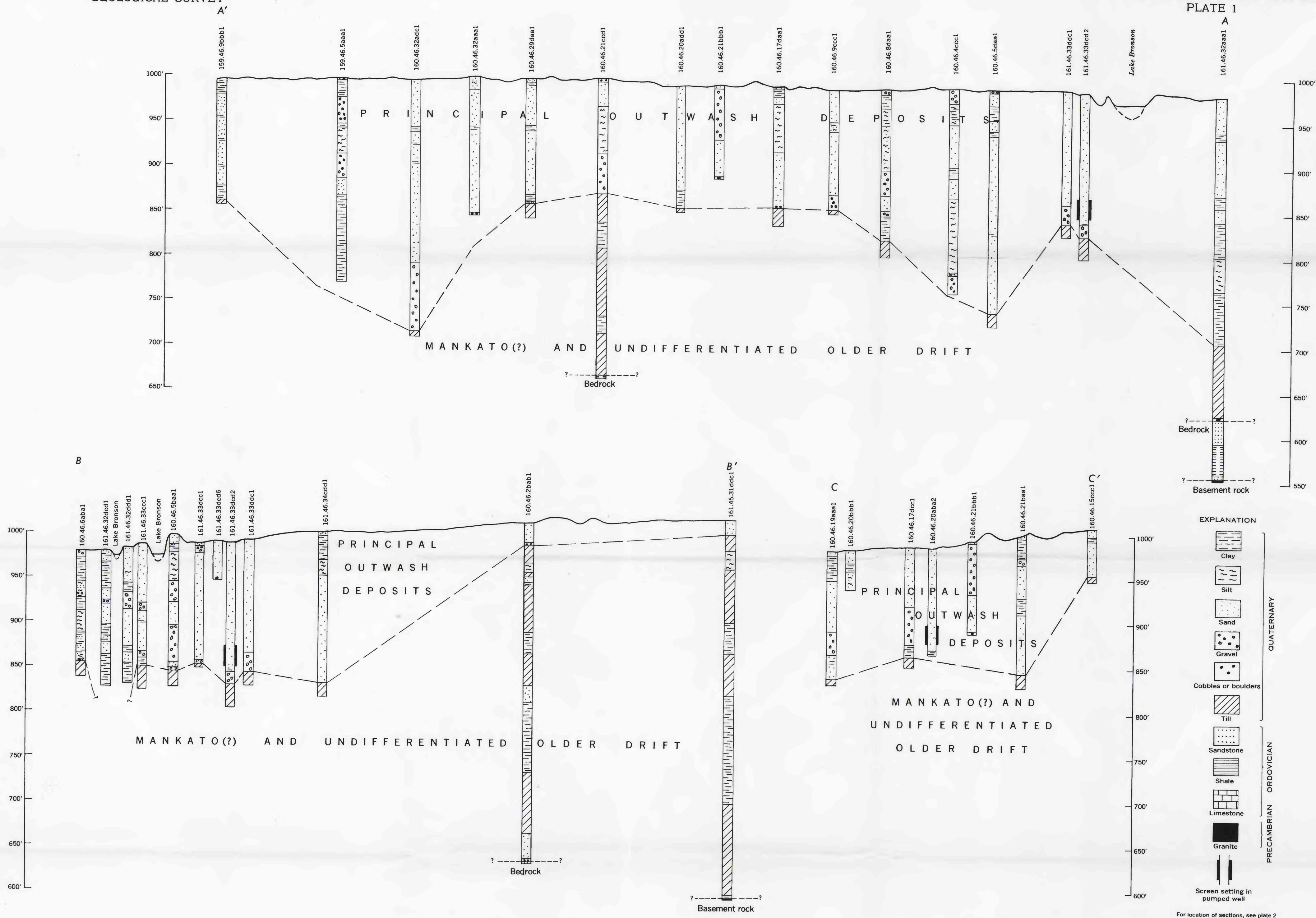
GEOLOGIC SECTIONS IN THE HALMA-LAKE BRONSON AREA, MINNESOTA, SHOWING LITHOLOGY AND DISTRIBUTION OF PRINCIPAL OUTWASH DEPOSITS
