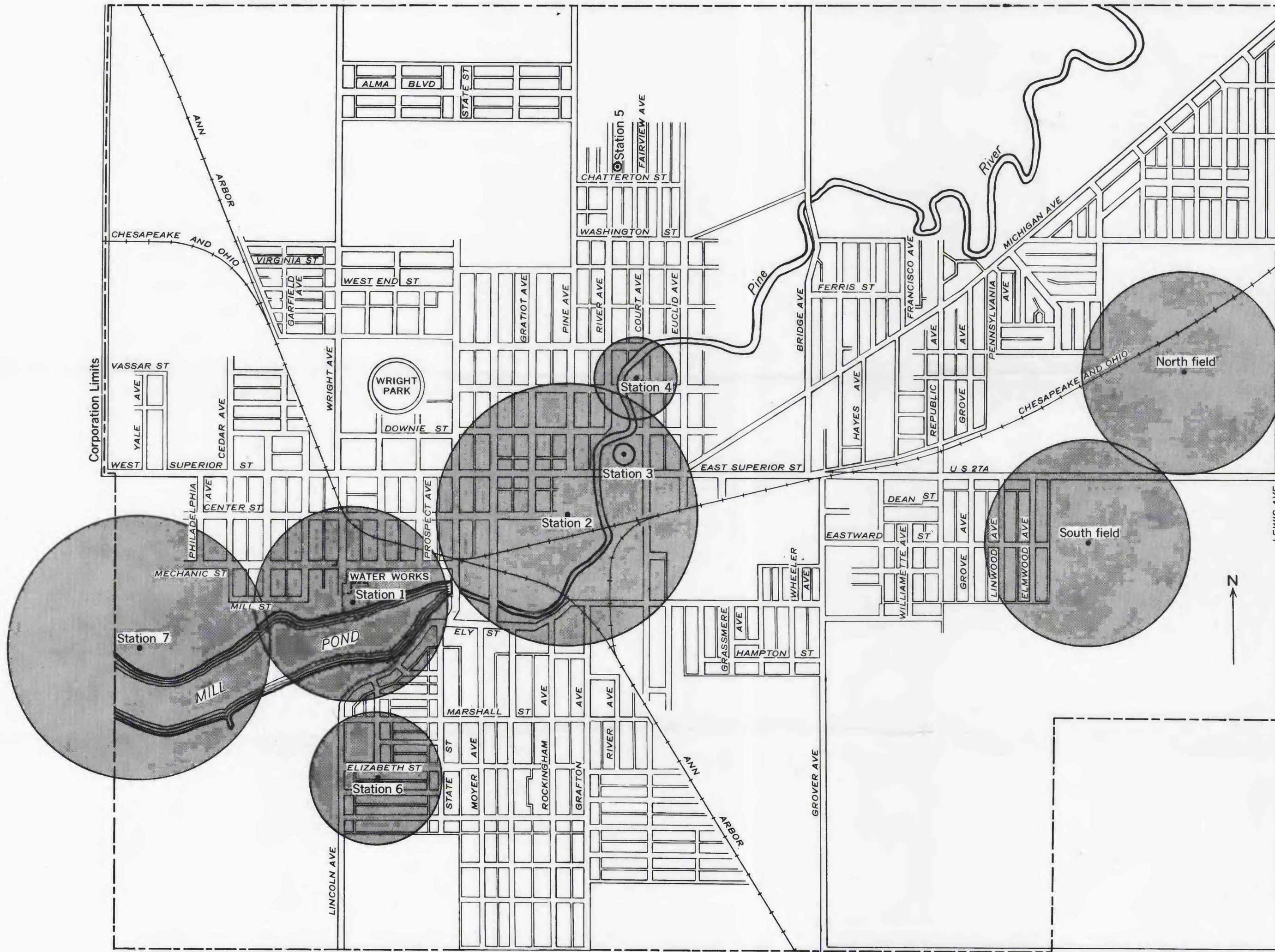
MAP OF THE CITY OF ALMA SHOWING PUMPAGE DISTRIBUTION AND MAGNITUDE IN 1959
