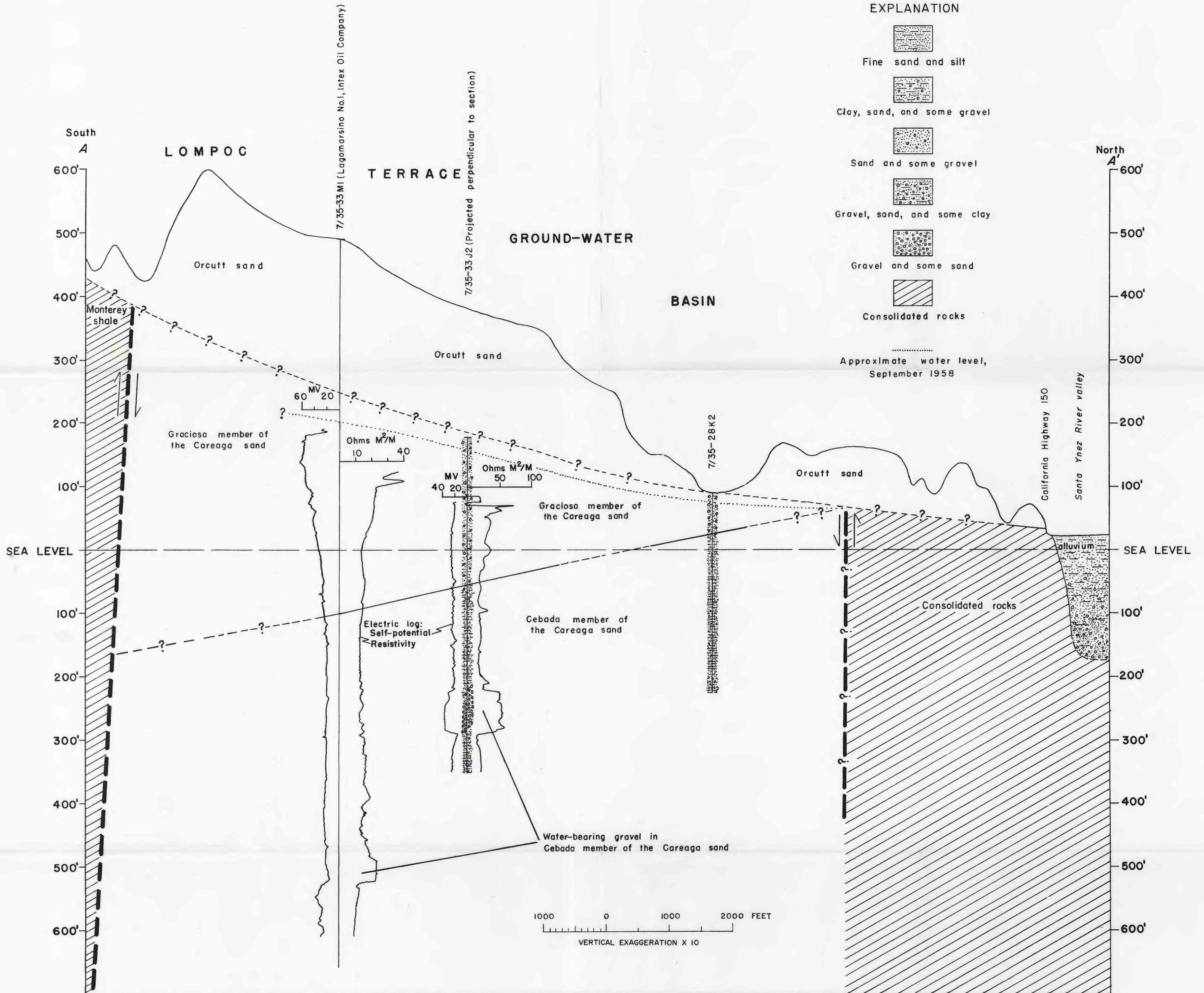
GENERALIZED GEOLOGIC SECTION A-A' THROUGH THE LOMPOC TERRACE GROUND-WATER BASIN, CALIFORNIA
